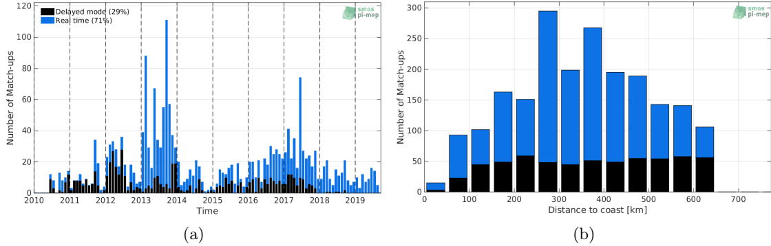
Figure 1: Number of match-ups between Argo and SMOS-L2-DPGS-v662 SSS as a function of time (a) and as function of the distance to coast (b) over the Bay of Bengal Pi-MEP region and for the full satellite product period.
