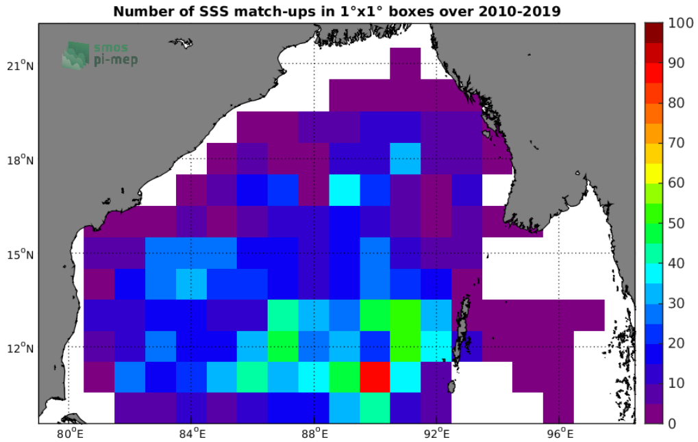
Figure 4: Number of SSS match-ups between Argo SSS and the SMOS-L2-DPGS-v662 SSS product for the Bay of Bengal Pi-MEP region over 1°x1° boxes and for the full satellite product period.
