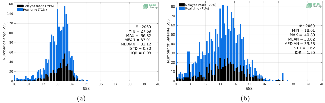
Figure 2: Histograms of SSS from Argo (a) and SMOS-L2-DPGS-v662 (b) considering all match-up pairs per bins of 0.1 over the Bay of Bengal Pi-MEP region and for the full satellite product period.
