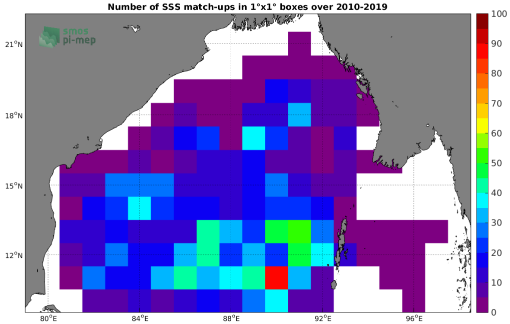
Figure 4: Number of SSS match-ups between Argo SSS and the SMOS-L2-DPGS-v662 SSS product for the Bay of Bengal Pi-MEP region over 1^\circ \times 1^\circ boxes and for the full satellite product period.
