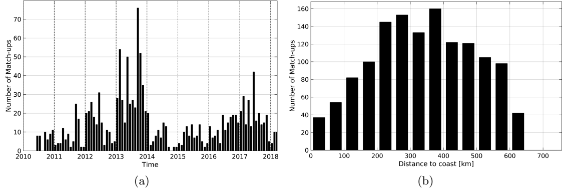
Figure 1: Number of match-ups between Argo and SMOS-L2-DPGS-v662 SSS as a function of time (a) and as function of the distance to coast (b) over the Bay of Bengal Pi-MEP region and for the full satellite product period.
