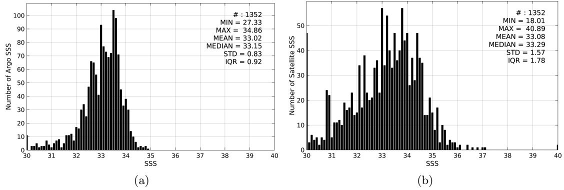
Figure 2: Histograms of SSS from Argo (a) and SMOS-L2-DPGS-v662 (b) considering all match-up pairs per bins of 0.1 over the Bay of Bengal Pi-MEP region and for the full satellite product period.
