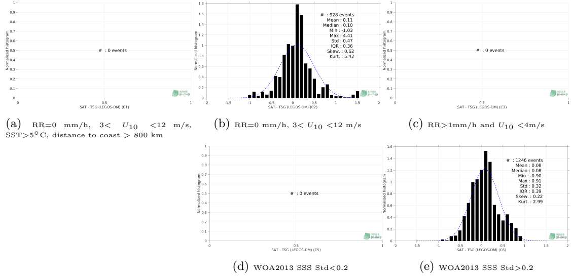
Figure 13: Normalized histogram of \Delta\text{SSS} (SMAP SSS L4 OI v1 - 7 Days (IPRC) - TSG (LEGOS-DM)) for 5 different subdatasets corresponding to: RR=0 mm/h, 3 < U_{10} < 12 m/s, SST > 5^\circ\text{C} , distance to coast > 800 km (a), RR=0 mm/h, 3 < U_{10} < 12 m/s (b), RR > 1\text{mm/h} and U_{10} < 4\text{m/s} (c), WOA2013 SSS Std < 0.2 (d), WOA2013 SSS Std > 0.2 (e).
