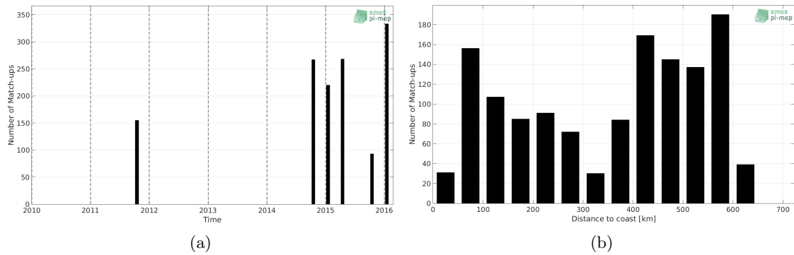
Figure 1: Number of match-ups between TSG (LEGOS-DM) and SMAP SSS L4 OI v1 - 7 Days (IPRC) SSS as a function of time (a) and as function of the distance to coast (b) over the Bay of Bengal Pi-MEP region and for the full satellite product period.
