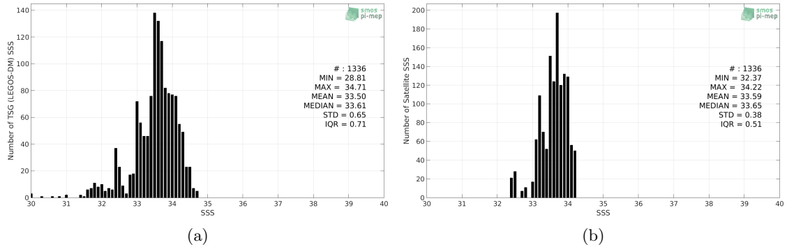
Figure 2: Histograms of SSS from TSG (LEGOS-DM) (a) and SMAP SSS L4 OI v1 - 7 Days (IPRC) (b) considering all match-up pairs per bins of 0.1 over the Bay of Bengal Pi-MEP region and for the full satellite product period.
