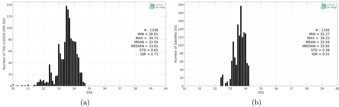
Figure 2: Histograms of SSS from TSG (LEGOS-DM) (a) and SMAP SSS L4 OI v1 - 7day (IPRC) (b) considering all match-up pairs per bins of 0.1 over the Bay of Bengal Pi-MEP region and for the full satellite product period.
