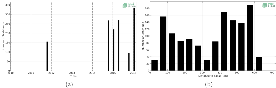
Figure 1: Number of match-ups between TSG (LEGOS-DM) and SMAP SSS L4 OI v1 - 7day (IPRC) SSS as a function of time (a) and as function of the distance to coast (b) over the Bay of Bengal Pi-MEP region and for the full satellite product period.
