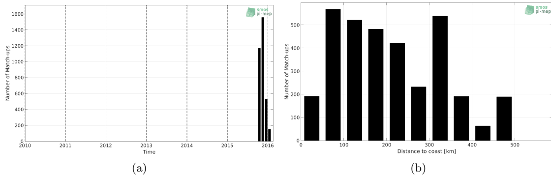
Figure 1: Number of match-ups between Surface drifters and SMAP SSS L4 OI v1 - 7 Days (IPRC) SSS as a function of time (a) and as function of the distance to coast (b) over the Bay of Bengal Pi-MEP region and for the full satellite product period.
