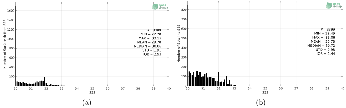
Figure 2: Histograms of SSS from Surface drifters (a) and SMAP SSS L4 OI v1 - 7 Days (IPRC) (b) considering all match-up pairs per bins of 0.1 over the Bay of Bengal Pi-MEP region and for the full satellite product period.
