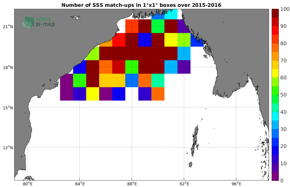
Figure 3: Number of SSS match-ups between Surface drifters SSS and the SMAP SSS L4 OI v1 - 7 Days (IPRC) SSS product for the Bay of Bengal Pi-MEP region over 1^\circ \times 1^\circ boxes and for the full satellite product period.
