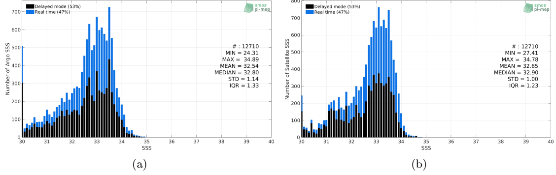
Figure 2: Histograms of SSS from Argo (a) and SMAP SSS L4 OI v1 - 7 Days (IPRC) (b) considering all match-up pairs per bins of 0.1 over the Bay of Bengal Pi-MEP region and for the full satellite product period.
