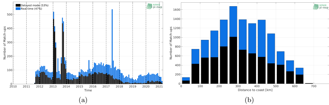
Figure 1: Number of match-ups between Argo and SMAP SSS L4 OI v1 - 7 Days (IPRC) SSS as a function of time (a) and as function of the distance to coast (b) over the Bay of Bengal Pi-MEP region and for the full satellite product period.
