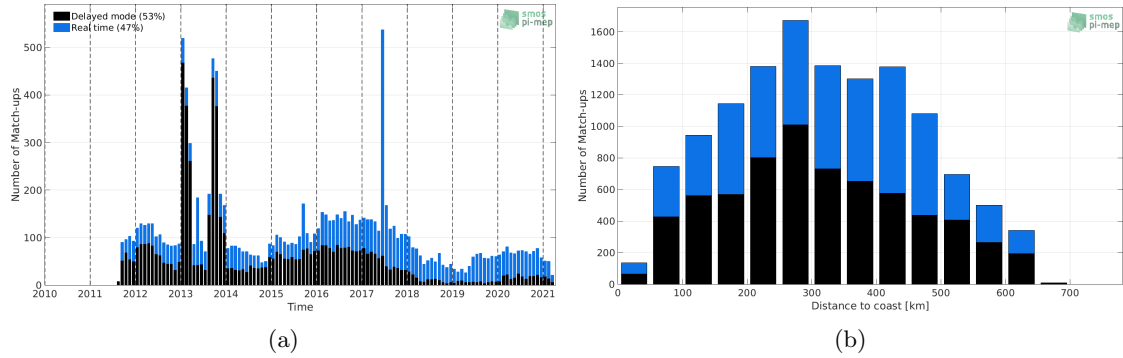
Figure 1: Number of match-ups between Argo and SMAP SSS L4 OI v1 - 7day (IPRC) SSS as a function of time (a) and as function of the distance to coast (b) over the Bay of Bengal Pi-MEP region and for the full satellite product period.
