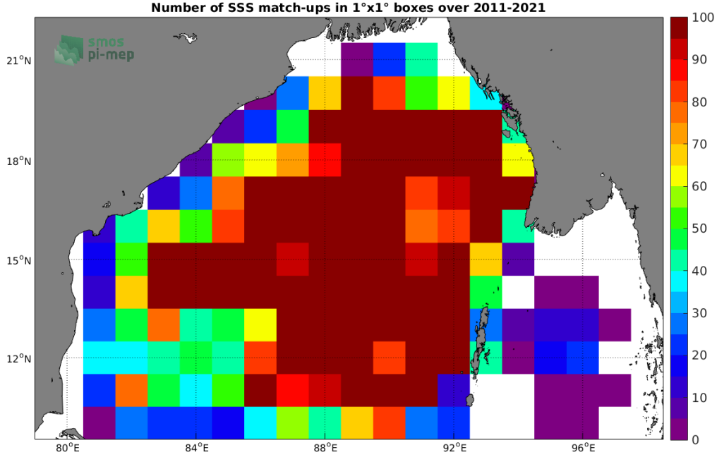
Figure 4: Number of SSS match-ups between Argo SSS and the SMAP SSS L4 OI v1 - 7day (IPRC) SSS product for the Bay of Bengal Pi-MEP region over 1^\circ \times 1^\circ boxes and for the full satellite product period.
