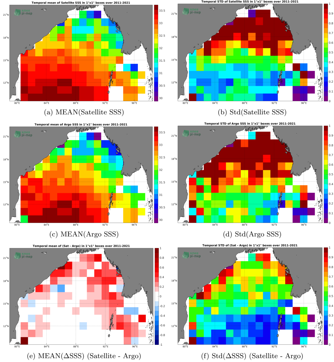
Figure 6: Temporal mean (left) and Std (right) of SSS from SMAP SSS L4 OI v1 - 7day (IPRC) (top), Argo (middle), and of \Delta SSS (Satellite - Argo). Only match-up pairs are used to generate these maps.
