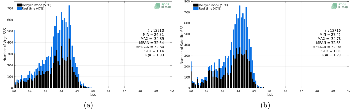
Figure 2: Histograms of SSS from Argo (a) and SMAP SSS L4 OI v1 - 7day (IPRC) (b) considering all match-up pairs per bins of 0.1 over the Bay of Bengal Pi-MEP region and for the full satellite product period.
