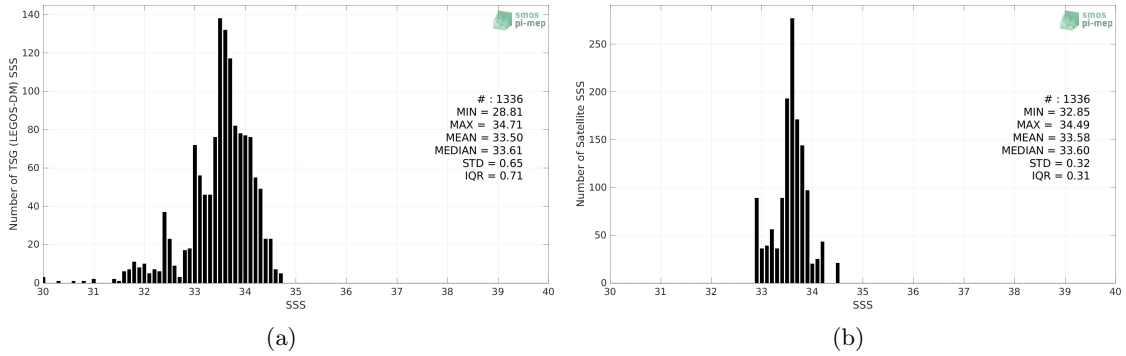
Figure 2: Histograms of SSS from TSG (LEGOS-DM) (a) and SMAP SSS L4 OI v1 - Monthly (IPRC) (b) considering all match-up pairs per bins of 0.1 over the Bay of Bengal Pi-MEP region and for the full satellite product period.
