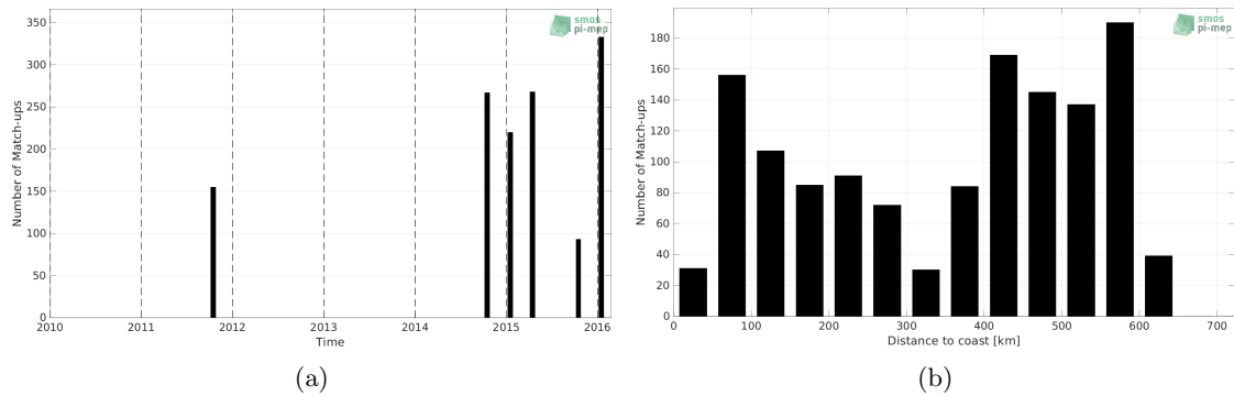
Figure 1: Number of match-ups between TSG (LEGOS-DM) and SMAP SSS L4 OI v1 - Monthly (IPRC) SSS as a function of time (a) and as function of the distance to coast (b) over the Bay of Bengal Pi-MEP region and for the full satellite product period.
