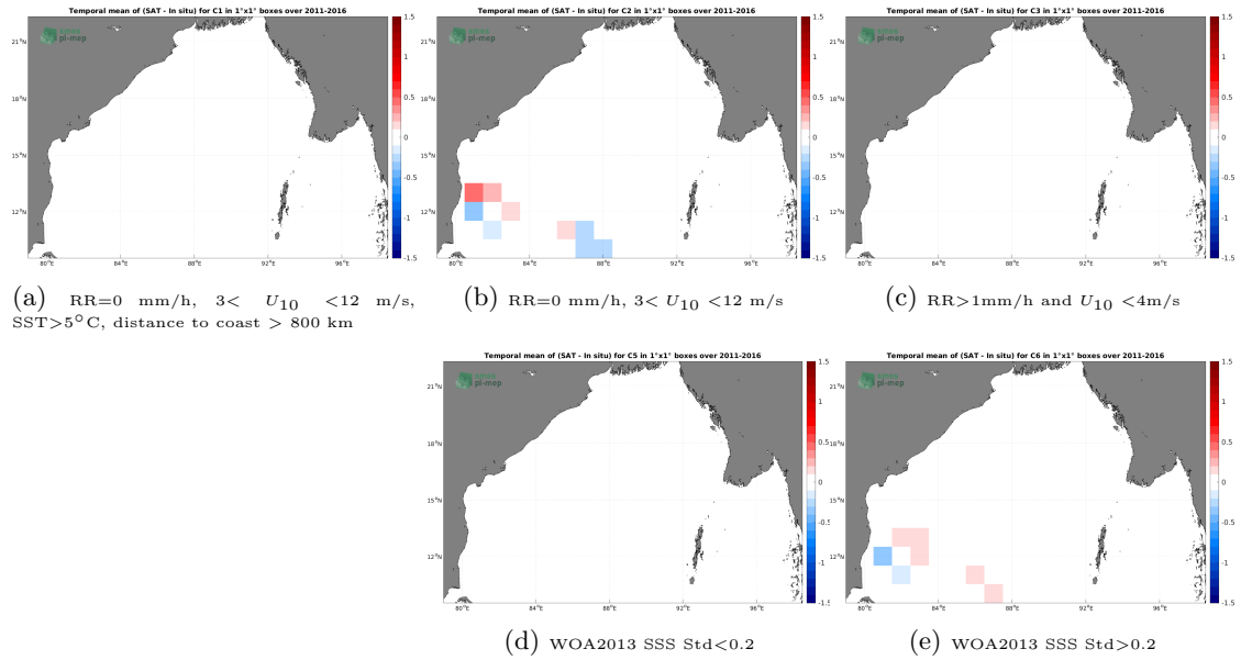
Figure 12: Temporal mean gridded over spatial boxes of size 1^\circ \times 1^\circ of \Delta SSS (SMAP SSS L4 OI v1 - Monthly (IPRC) - TSG (LEGOS-DM)) for 5 different subdatasets corresponding to:RR=0 mm/h, 3 < U_{10} < 12 m/s, SST > 5^\circ\text{C} , distance to coast > 800 km (a), RR=0 mm/h, 3 < U_{10} < 12 m/s (b), RR > 1 mm/h and U_{10} < 4 m/s (c), WOA2013 SSS Std < 0.2 (d), WOA2013 SSS Std > 0.2 (e).
