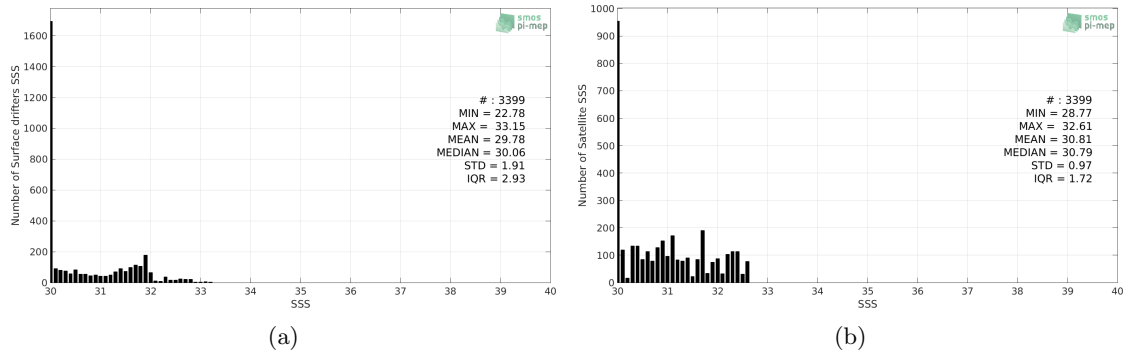
Figure 2: Histograms of SSS from Surface drifters (a) and SMAP SSS L4 OI v1 - Monthly (IPRC) (b) considering all match-up pairs per bins of 0.1 over the Bay of Bengal Pi-MEP region and for the full satellite product period.
