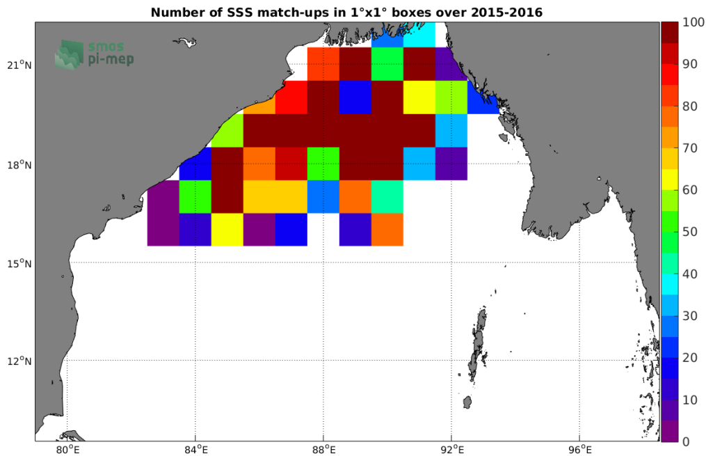
Figure 3: Number of SSS match-ups between Surface drifters SSS and the SMAP SSS L4 OI v1 - Monthly (IPRC) SSS product for the Bay of Bengal Pi-MEP region over 1^\circ \times 1^\circ boxes and for the full satellite product period.
