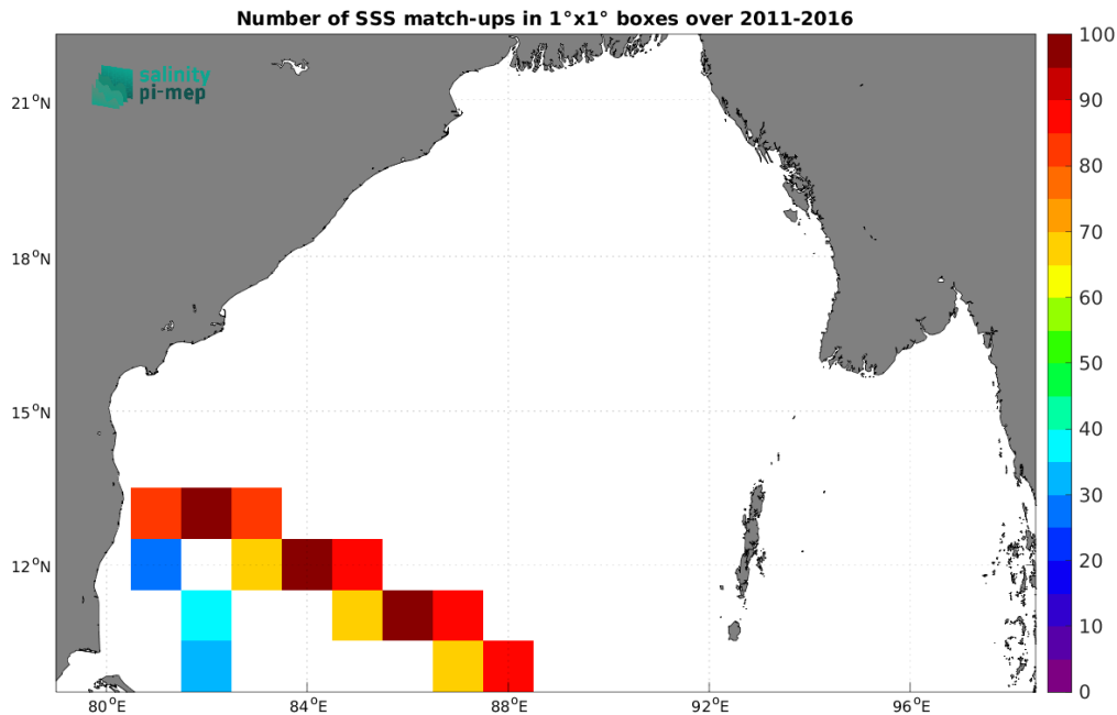
Figure 5: Number of SSS match-ups between TSG (LEGOS-DM) SSS and the SMAP SSS L4 OI v3 - Monthly (ESR) SSS product for the Bay of Bengal Pi-MEP region over 1^\circ \times 1^\circ boxes and for the full satellite product period.
