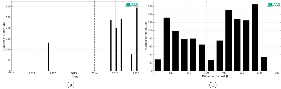
Figure 2: Number of match-ups between TSG (LEGOS-DM) and SMAP SSS L4 OI v3 - Monthly (ESR) SSS as a function of time (a) and as function of the distance to coast (b) over the Bay of Bengal Pi-MEP region and for the full satellite product period.
