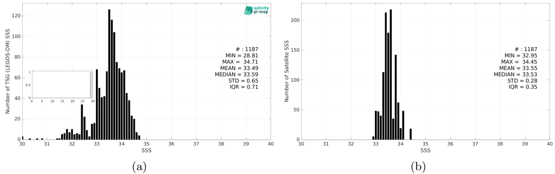
Figure 3: Histograms of SSS from TSG (LEGOS-DM) (a) and SMAP SSS L4 OI v3 - Monthly (ESR) (b) considering all match-up pairs per bins of 0.1 over the Bay of Bengal Pi-MEP region and for the full satellite product period.
