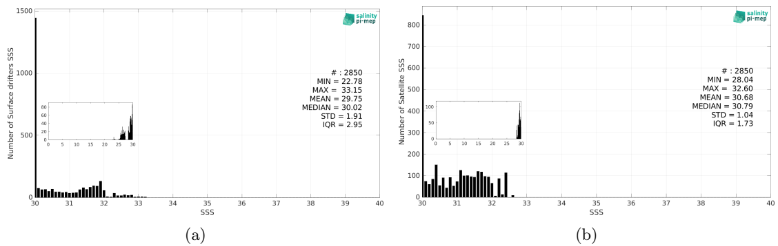
Figure 3: Histograms of SSS from Surface drifters (a) and SMAP SSS L4 OI v3 - Monthly (ESR) (b) considering all match-up pairs per bins of 0.1 over the Bay of Bengal Pi-MEP region and for the full satellite product period.
