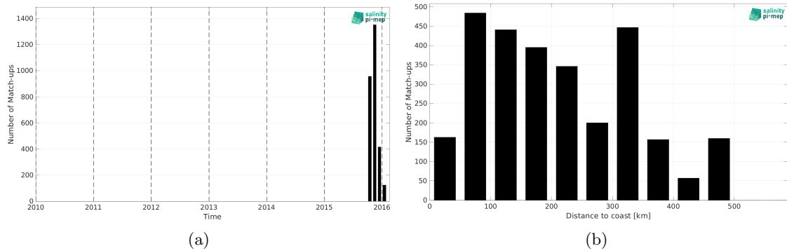
Figure 2: Number of match-ups between Surface drifters and SMAP SSS L4 OI v3 - Monthly (ESR) SSS as a function of time (a) and as function of the distance to coast (b) over the Bay of Bengal Pi-MEP region and for the full satellite product period.
