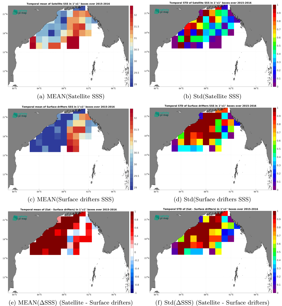
Figure 6: Temporal mean (left) and Std (right) of SSS from SMAP SSS L4 OI v3 - Monthly (ESR) (top), Surface drifters (middle), and of \Delta SSS (Satellite - Surface drifters). Only match-up pairs are used to generate these maps.
