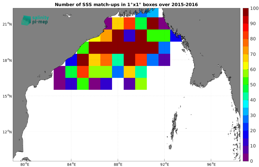
Figure 4: Number of SSS match-ups between Surface drifters SSS and the SMAP SSS L4 OI v3 - Monthly (ESR) SSS product for the Bay of Bengal Pi-MEP region over 1^\circ \times 1^\circ boxes and for the full satellite product period.
