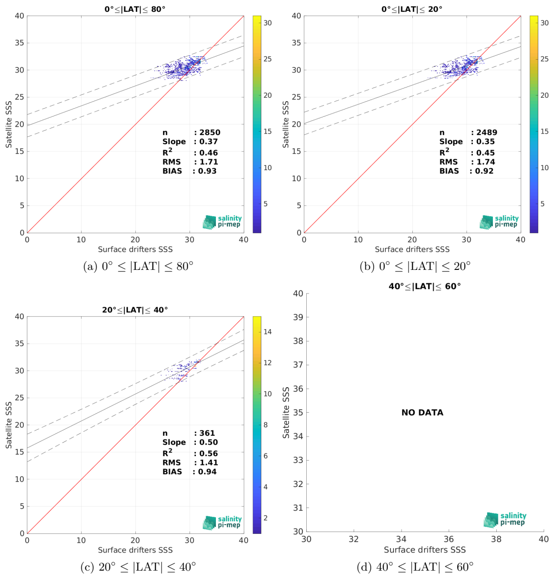
Figure 9: Contour maps of the concentration of SMAP SSS L4 OI v3 - Monthly (ESR) SSS (y-axis) versus Surface drifters SSS (x-axis) at match-up pairs for different latitude bands. For each plot, the red line shows x=y . The black thin and dashed lines indicate a linear fit through the data cloud and the \pm 95\% confidence levels, respectively. The number match-up pairs n , the slope and R^2 coefficient of the linear fit, the root mean square (RMS) and the mean bias between satellite and in situ data are indicated for each latitude band in each plots.
