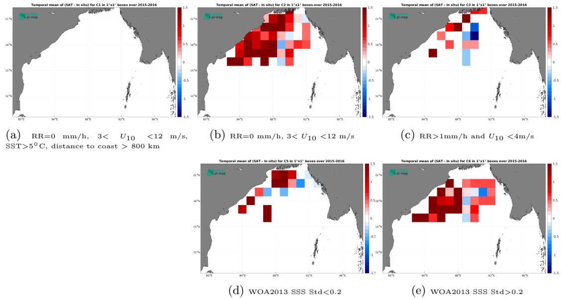
Figure 13: Temporal mean gridded over spatial boxes of size 1^\circ \times 1^\circ of \Delta SSS (SMAP SSS L4 OI v3 - Monthly (ESR) - Surface drifters) for 5 different subdatasets corresponding to:RR=0 mm/h, 3 < U_{10} < 12 m/s, SST > 5^\circ\text{C} , distance to coast > 800 km (a), RR=0 mm/h, 3 < U_{10} < 12 m/s (b), RR > 1 mm/h and U_{10} < 4 m/s (c), WOA2013 SSS Std < 0.2 (d), WOA2013 SSS Std > 0.2 (e).
