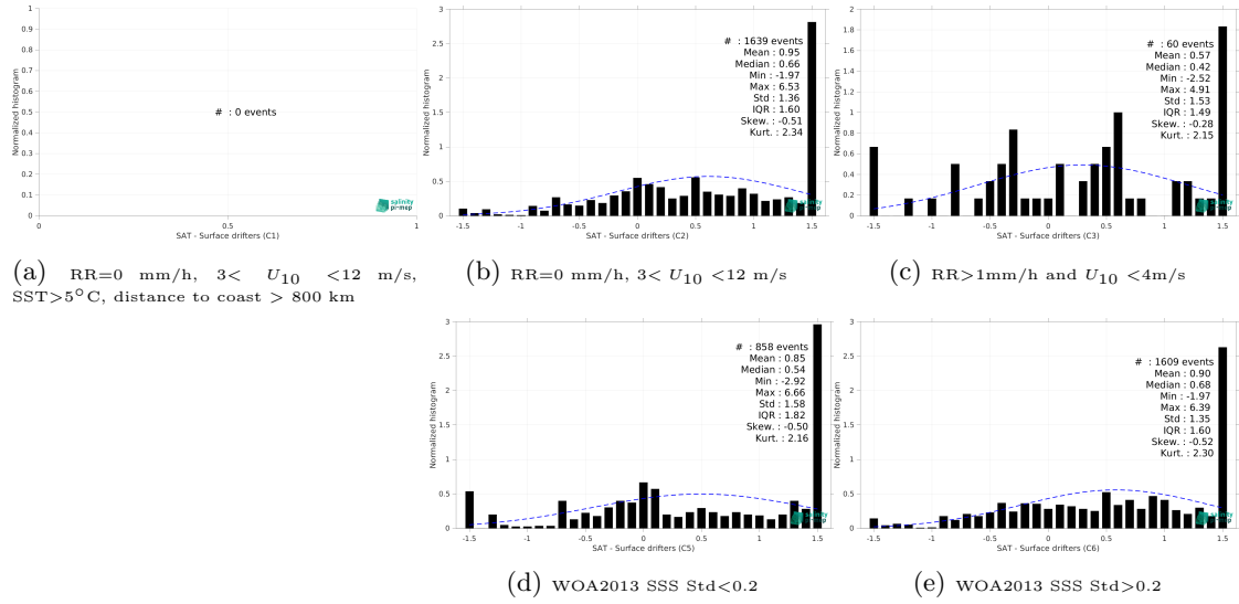
Figure 14: Normalized histogram of \Delta SSS (SMAP SSS L4 OI v3 - Monthly (ESR) - Surface drifters) for 5 different subdatasets corresponding to: RR=0 mm/h, 3 < U_{10} < 12 m/s, SST > 5°C, distance to coast > 800 km (a), RR=0 mm/h, 3 < U_{10} < 12 m/s (b), RR > 1mm/h and U_{10} < 4 m/s (c), WOA2013 SSS Std < 0.2 (d), WOA2013 SSS Std > 0.2 (e).
