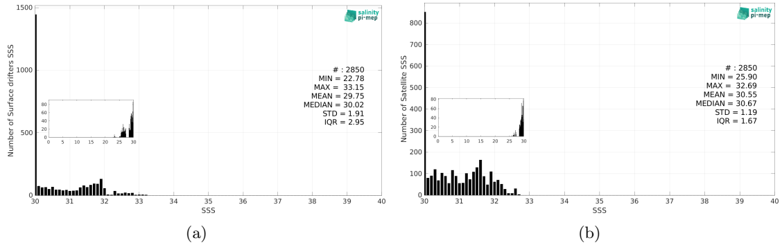
Figure 3: Histograms of SSS from Surface drifters (a) and SMAP SSS L4 OI v3 - Daily (ESR) (b) considering all match-up pairs per bins of 0.1 over the Bay of Bengal Pi-MEP region and for the full satellite product period.
