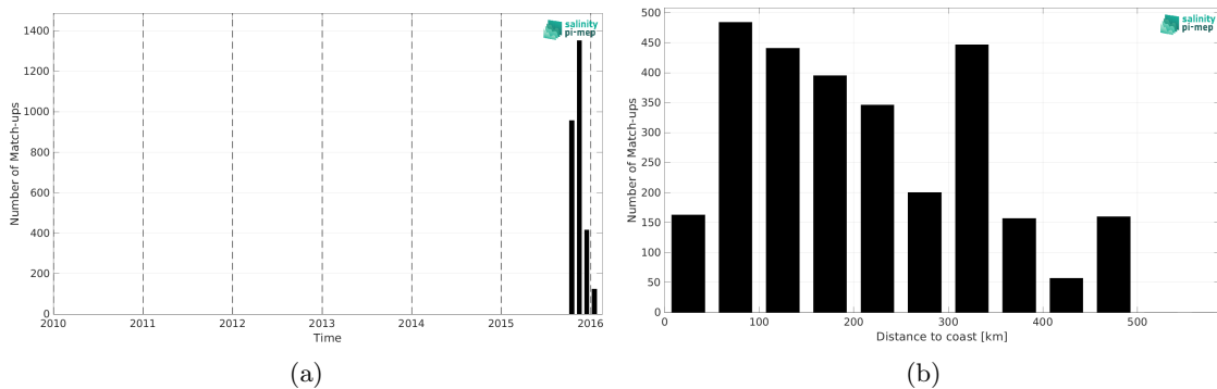
Figure 2: Number of match-ups between Surface drifters and SMAP SSS L4 OI v3 - Daily (ESR) SSS as a function of time (a) and as function of the distance to coast (b) over the Bay of Bengal Pi-MEP region and for the full satellite product period.
