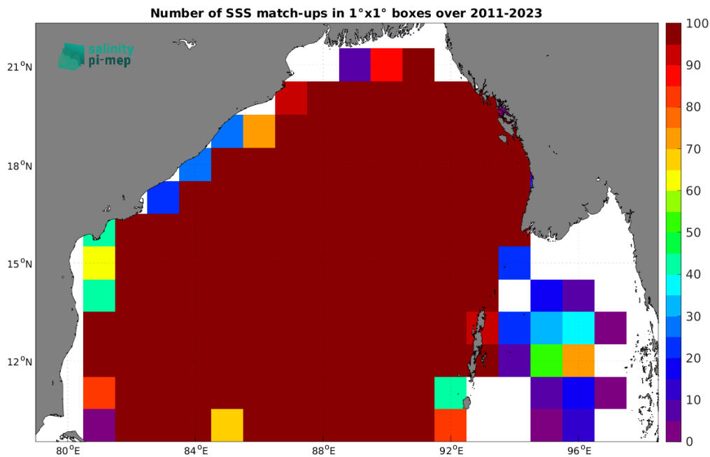
Figure 5: Number of SSS match-ups between Argo SSS and the SMAP SSS L4 OI v3 - Daily (ESR) SSS product for the Bay of Bengal Pi-MEP region over 1^\circ \times 1^\circ boxes and for the full satellite product period.
