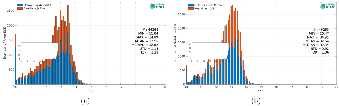
Figure 3: Histograms of SSS from Argo (a) and SMAP SSS L4 OI v3 - Daily (ESR) (b) considering all match-up pairs per bins of 0.1 over the Bay of Bengal Pi-MEP region and for the full satellite product period.
