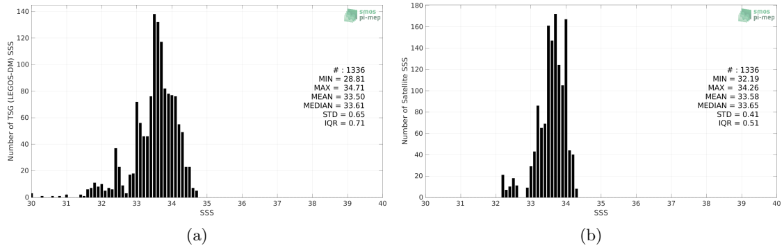
Figure 2: Histograms of SSS from TSG (LEGOS-DM) (a) and SMAP SSS L4 OI v2 - 7 Days (ESR) (b) considering all match-up pairs per bins of 0.1 over the Bay of Bengal Pi-MEP region and for the full satellite product period.
