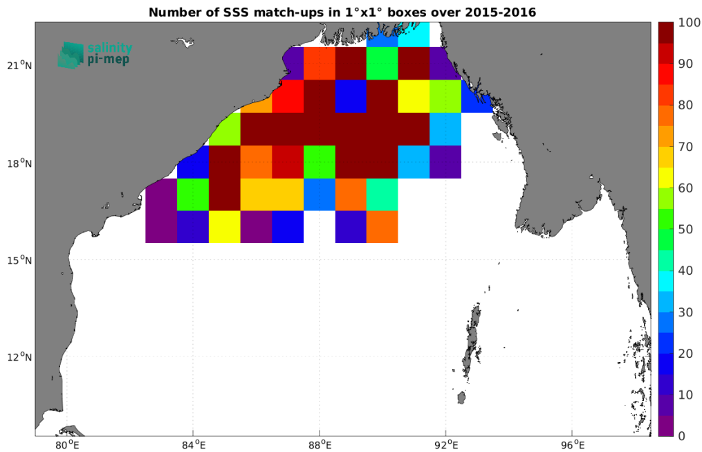
Figure 3: Number of SSS match-ups between Surface drifters SSS and the SMAP SSS L4 OI v2 - 7 Days (ESR) SSS product for the Bay of Bengal Pi-MEP region over 1^\circ \times 1^\circ boxes and for the full satellite product period.
