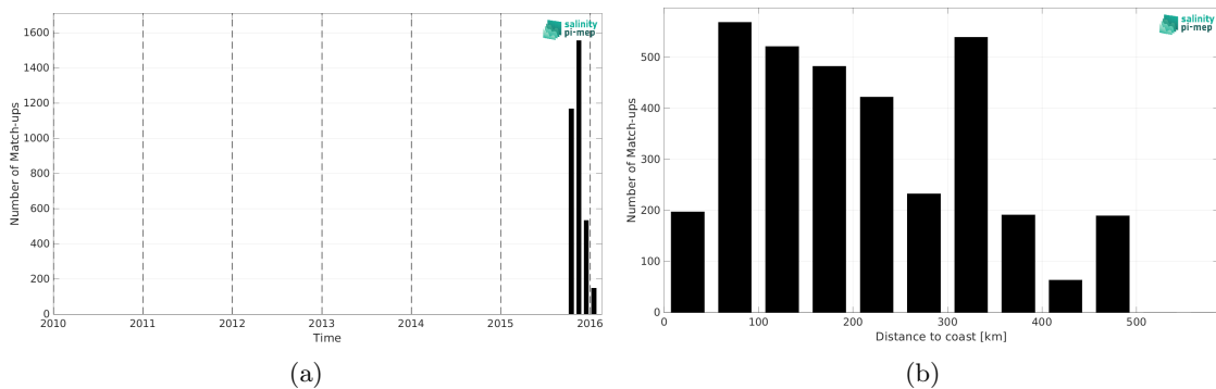
Figure 1: Number of match-ups between Surface drifters and SMAP SSS L4 OI v2 - 7 Days (ESR) SSS as a function of time (a) and as function of the distance to coast (b) over the Bay of Bengal Pi-MEP region and for the full satellite product period.
