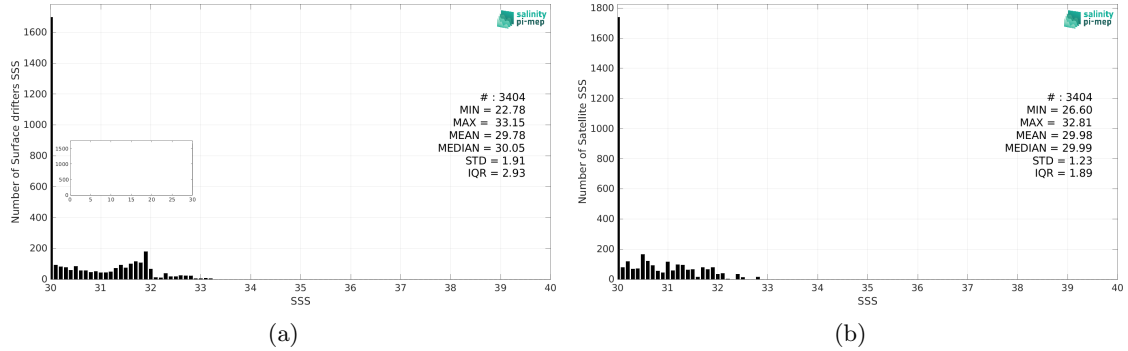
Figure 2: Histograms of SSS from Surface drifters (a) and SMAP SSS L4 OI v2 - 7 Days (ESR) (b) considering all match-up pairs per bins of 0.1 over the Bay of Bengal Pi-MEP region and for the full satellite product period.
