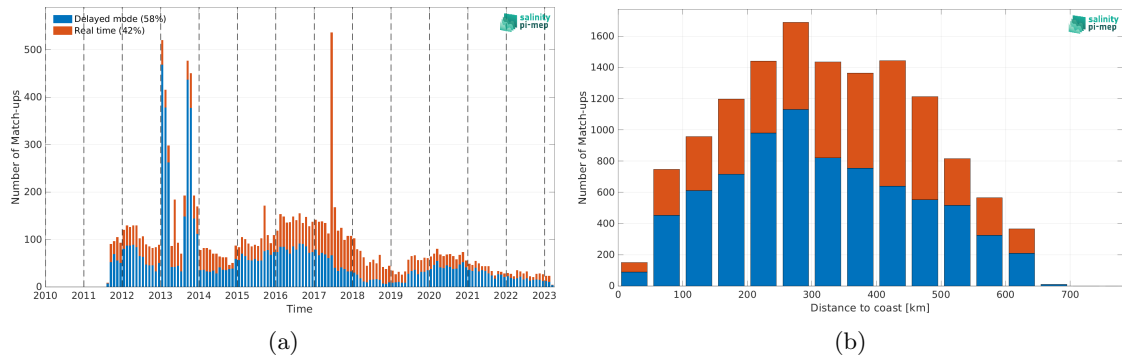
Figure 1: Number of match-ups between Argo and SMAP SSS L4 OI v2 - 7 Days (ESR) SSS as a function of time (a) and as function of the distance to coast (b) over the Bay of Bengal Pi-MEP region and for the full satellite product period.
