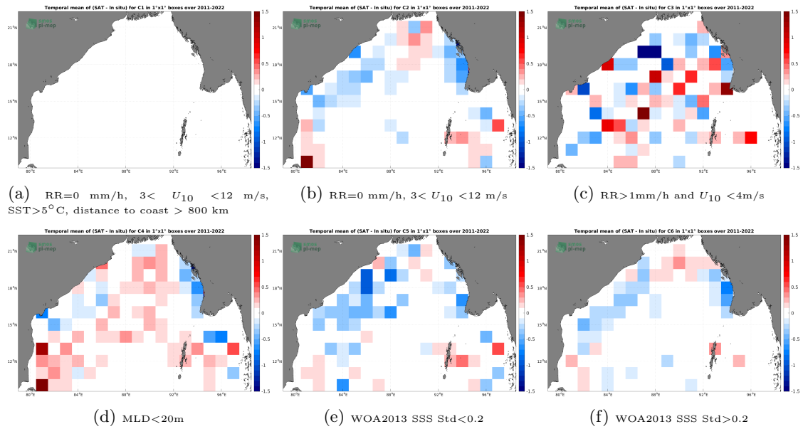
Figure 12: Temporal mean gridded over spatial boxes of size 1^\circ \times 1^\circ of \Delta SSS (SMAP SSS L4 OI v2 - 7 Days (ESR) - Argo) for 6 different subdatasets corresponding to: RR=0 mm/h, 3 < U_{10} < 12 m/s, SST > 5^\circ\text{C} , distance to coast > 800 km (a), RR=0 mm/h, 3 < U_{10} < 12 m/s (b), RR > 1 mm/h and U_{10} < 4 m/s (c), MLD < 20 m (d), WOA2013 SSS Std < 0.2 (e), WOA2013 SSS Std > 0.2 (f).
