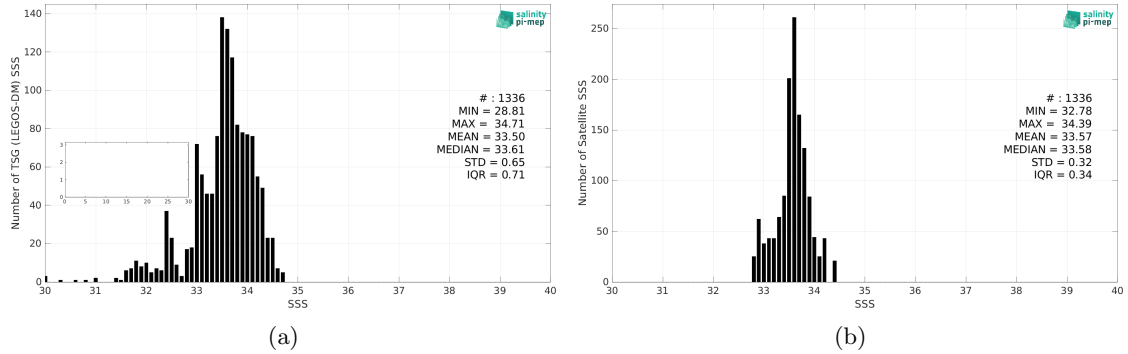
Figure 2: Histograms of SSS from TSG (LEGOS-DM) (a) and SMAP SSS L4 OI v2 - Monthly (IPRC) (b) considering all match-up pairs per bins of 0.1 over the Bay of Bengal Pi-MEP region and for the full satellite product period.
