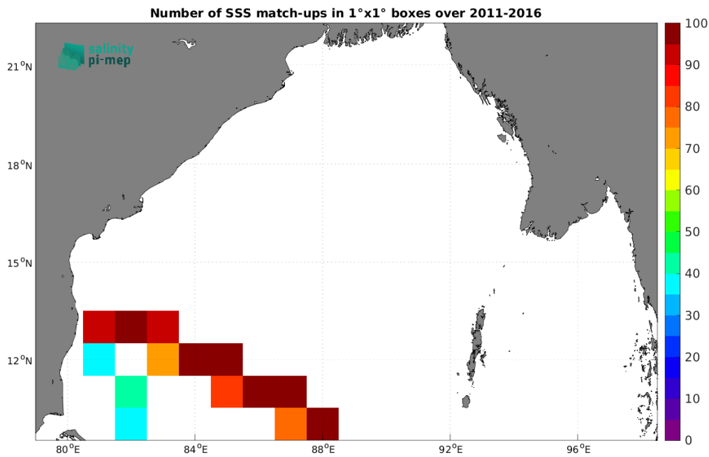
Figure 4: Number of SSS match-ups between TSG (LEGOS-DM) SSS and the SMAP SSS L4 OI v2 - Monthly (IPRC) SSS product for the Bay of Bengal Pi-MEP region over 1^\circ \times 1^\circ boxes and for the full satellite product period.
