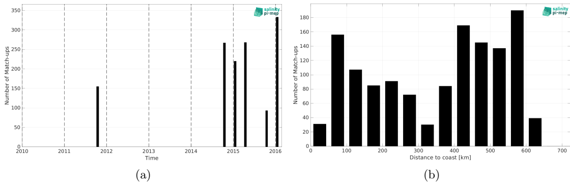
Figure 1: Number of match-ups between TSG (LEGOS-DM) and SMAP SSS L4 OI v2 - Monthly (IPRC) SSS as a function of time (a) and as function of the distance to coast (b) over the Bay of Bengal Pi-MEP region and for the full satellite product period.
