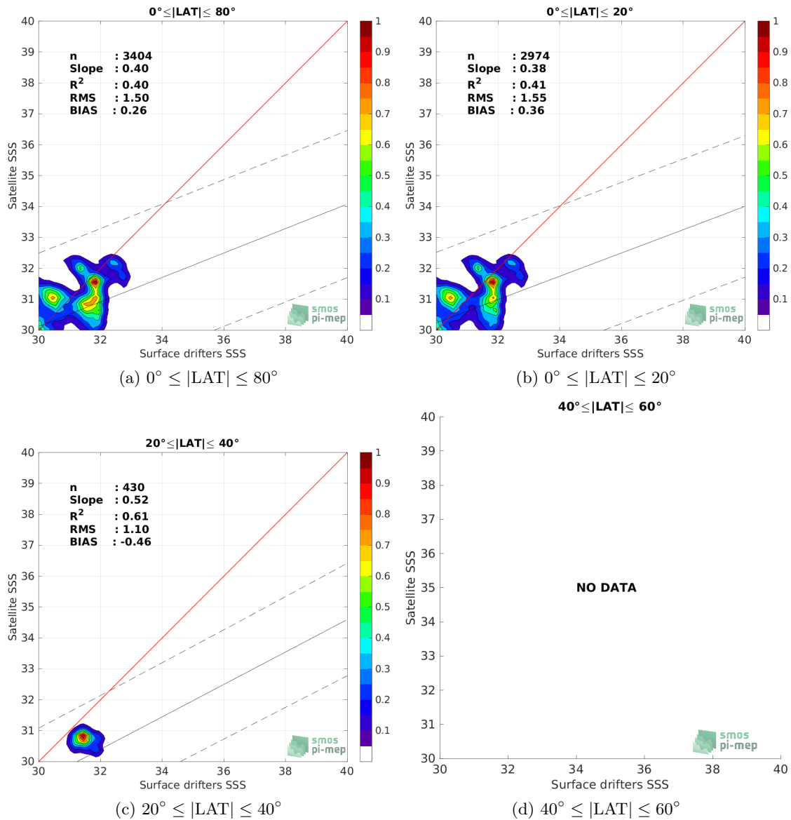
Figure 8: Contour maps of the concentration of SMAP SSS L4 OI v2 - Monthly (IPRC) SSS (y-axis) versus Surface drifters SSS (x-axis) at match-up pairs for different latitude bands. For each plot, the red line shows x=y . The black thin and dashed lines indicate a linear fit through the data cloud and the \pm 95\% confidence levels, respectively. The number match-up pairs n , the slope and R^2 coefficient of the linear fit, the root mean square (RMS) and the mean bias between satellite and in situ data are indicated for each latitude band in each plots.
