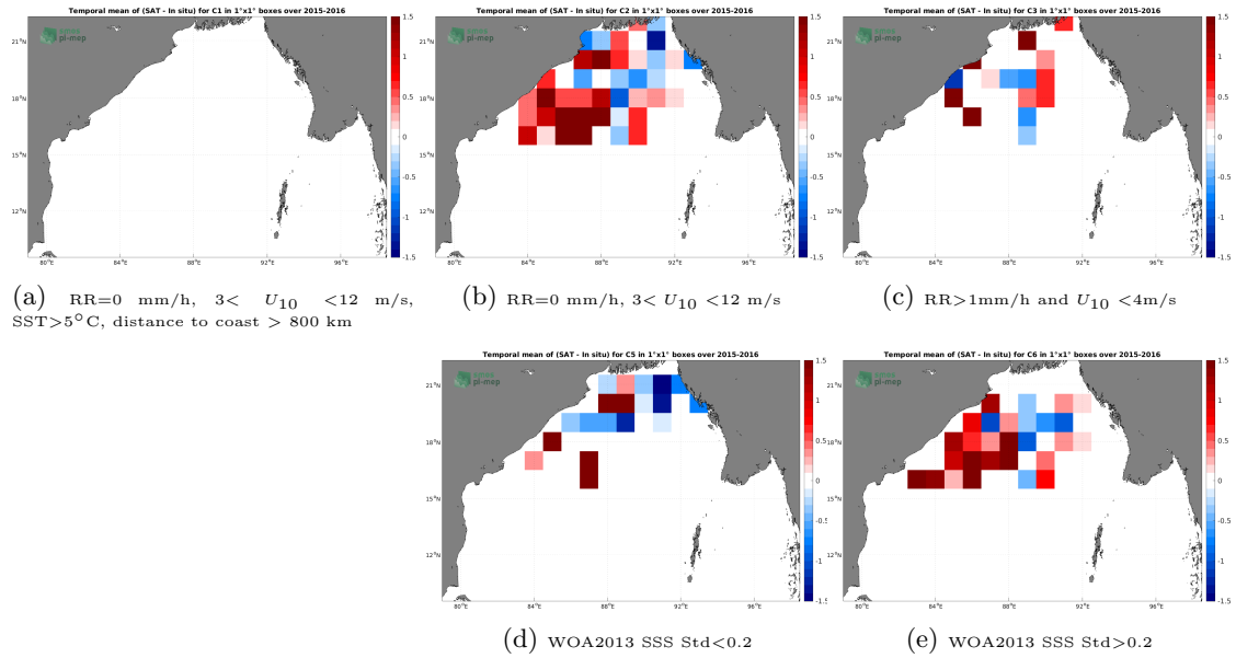
Figure 11: Temporal mean gridded over spatial boxes of size 1^\circ \times 1^\circ of \Delta SSS (SMAP SSS L4 OI v2 - Monthly (IPRC) - Surface drifters) for 5 different subdatasets corresponding to:RR=0 mm/h, 3 < U_{10} < 12 m/s, SST > 5^\circ\text{C} , distance to coast > 800 km (a), RR=0 mm/h, 3 < U_{10} < 12 m/s (b), RR > 1 mm/h and U_{10} < 4 m/s (c), WOA2013 SSS Std < 0.2 (d), WOA2013 SSS Std > 0.2 (e).
