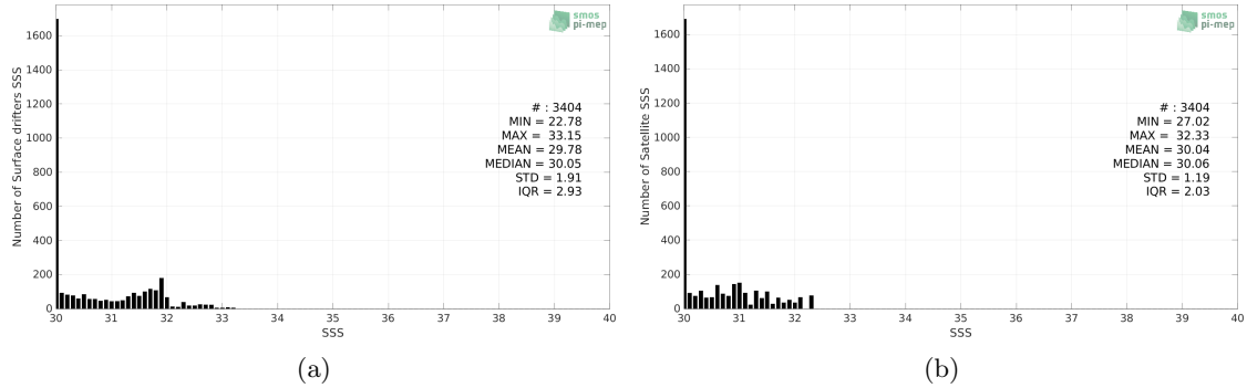
Figure 2: Histograms of SSS from Surface drifters (a) and SMAP SSS L4 OI v2 - Monthly (IPRC) (b) considering all match-up pairs per bins of 0.1 over the Bay of Bengal Pi-MEP region and for the full satellite product period.
