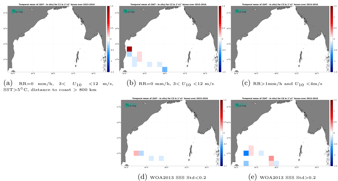
Figure 14: Temporal mean gridded over spatial boxes of size 1^\circ \times 1^\circ of \Delta\text{SSS} (SMAP SSS L3 v6 - 8-Day running (RSS) - TSG (LEGOS-DM)) for 5 different subdatasets corresponding to:RR=0 mm/h, 3 < U_{10} < 12 m/s, SST >5^\circ\text{C} , distance to coast > 800 km (a), RR=0 mm/h, 3 < U_{10} < 12 m/s (b), RR >1 mm/h and U_{10} < 4 m/s (c), WOA2013 SSS Std <0.2 (d), WOA2013 SSS Std >0.2 (e).
