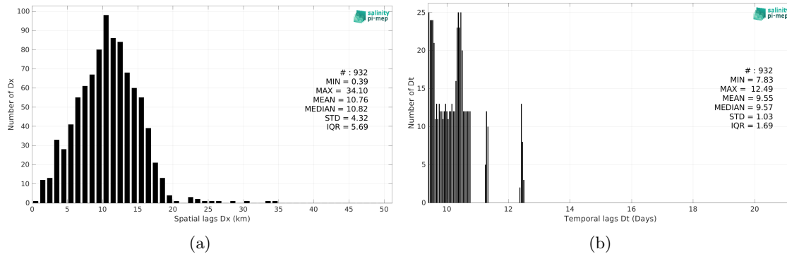
Figure 6: Histograms of the spatial (a) and temporal (b) lags between the location/time of the TSG (LEGOS-DM) measurement and the date of the corresponding SMAP SSS L3 v6 - Monthly (RSS) SSS pixel.
