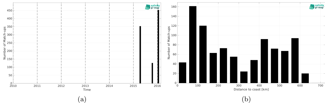
Figure 2: Number of match-ups between TSG (LEGOS-DM) and SMAP SSS L3 v6 - Monthly (RSS) SSS as a function of time (a) and as function of the distance to coast (b) over the Bay of Bengal Pi-MEP region and for the full satellite product period.
