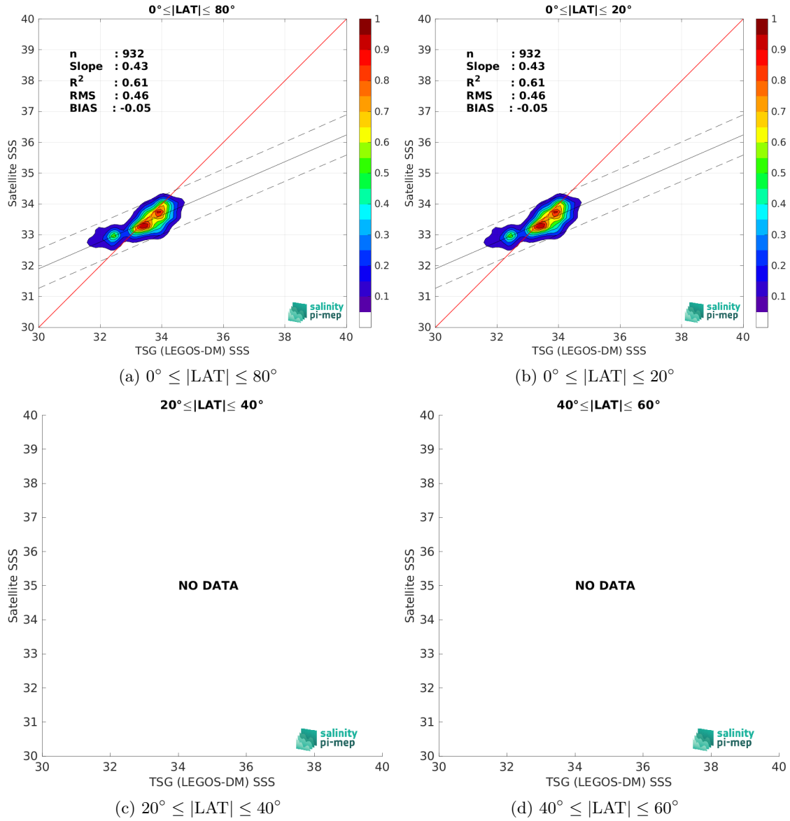
Figure 10: Contour maps of the concentration of SMAP SSS L3 v6 - Monthly (RSS) SSS (y-axis) versus TSG (LEGOS-DM) SSS (x-axis) at match-up pairs for different latitude bands. For each plot, the red line shows x=y . The black thin and dashed lines indicate a linear fit through the data cloud and the \pm 95\% confidence levels, respectively. The number match-up pairs n , the slope and R^2 coefficient of the linear fit, the root mean square (RMS) and the mean bias between satellite and in situ data are indicated for each latitude band in each plots.
