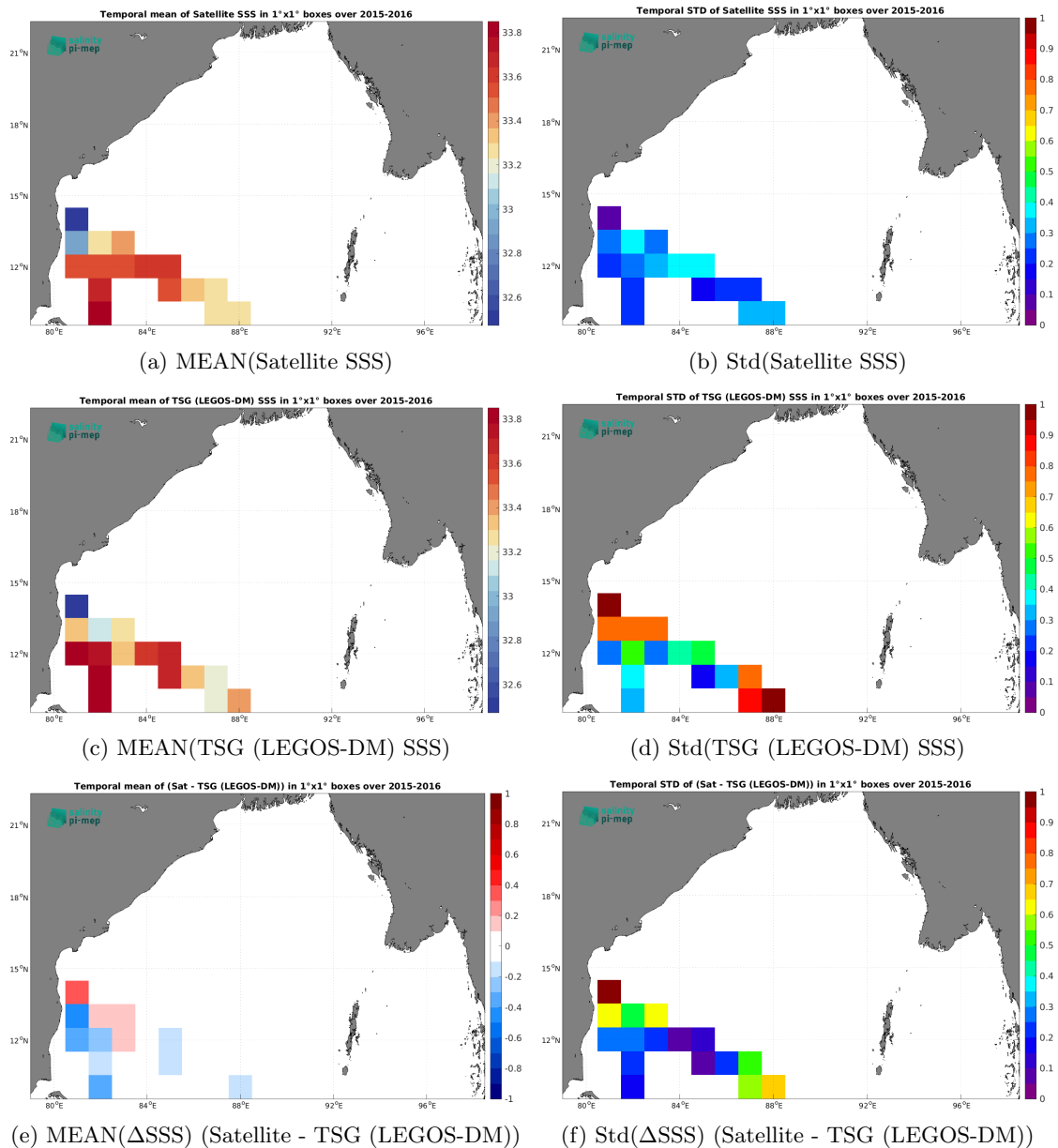
Figure 7: Temporal mean (left) and Std (right) of SSS from SMAP SSS L3 v6 - Monthly (RSS) (top), TSG (LEGOS-DM) (middle), and of \Delta SSS (Satellite - TSG (LEGOS-DM)). Only match-up pairs are used to generate these maps.
