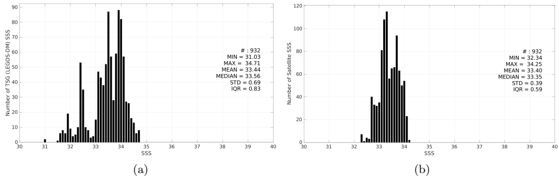
Figure 3: Histograms of SSS from TSG (LEGOS-DM) (a) and SMAP SSS L3 v6 - Monthly (RSS) (b) considering all match-up pairs per bins of 0.1 over the Bay of Bengal Pi-MEP region and for the full satellite product period.
