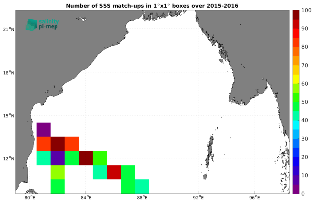
Figure 5: Number of SSS match-ups between TSG (LEGOS-DM) SSS and the SMAP SSS L3 v5.3 - 8-Day running (RSS) SSS product for the Bay of Bengal Pi-MEP region over 1^\circ \times 1^\circ boxes and for the full satellite product period.
