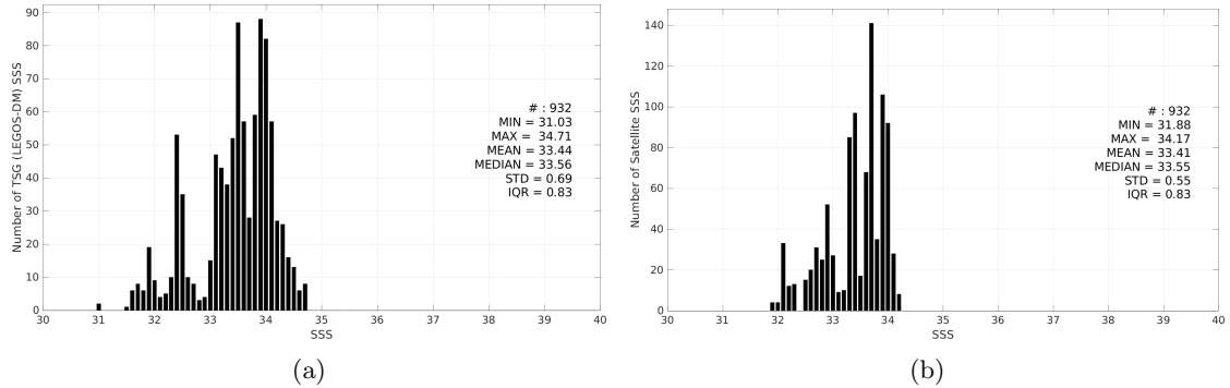
Figure 3: Histograms of SSS from TSG (LEGOS-DM) (a) and SMAP SSS L3 v5.3 - 8-Day running (RSS) (b) considering all match-up pairs per bins of 0.1 over the Bay of Bengal Pi-MEP region and for the full satellite product period.
