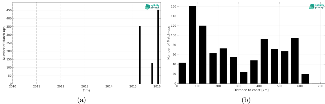
Figure 2: Number of match-ups between TSG (LEGOS-DM) and SMAP SSS L3 v5.3 - 8-Day running (RSS) SSS as a function of time (a) and as function of the distance to coast (b) over the Bay of Bengal Pi-MEP region and for the full satellite product period.
