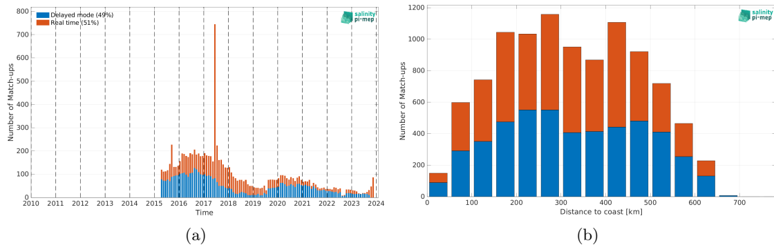
Figure 2: Number of match-ups between Argo and SMAP SSS L3 v5.3 - 8-Day running (RSS) SSS as a function of time (a) and as function of the distance to coast (b) over the Bay of Bengal Pi-MEP region and for the full satellite product period.
