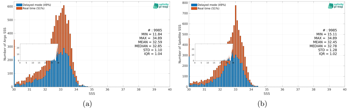
Figure 3: Histograms of SSS from Argo (a) and SMAP SSS L3 v5.3 - 8-Day running (RSS) (b) considering all match-up pairs per bins of 0.1 over the Bay of Bengal Pi-MEP region and for the full satellite product period.
