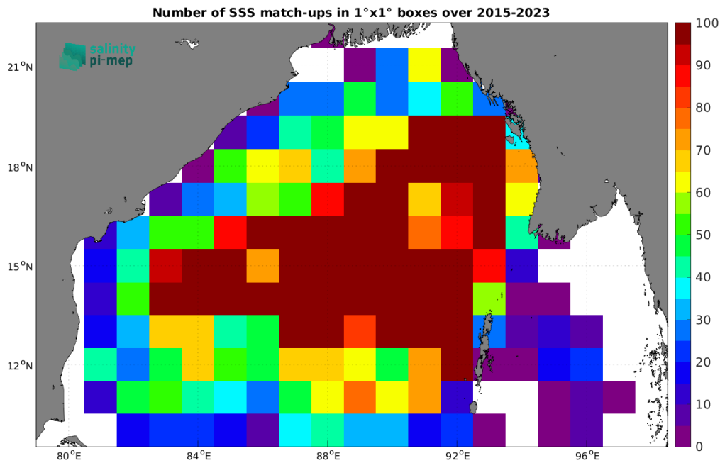
Figure 5: Number of SSS match-ups between Argo SSS and the SMAP SSS L3 v5.3 - 8-Day running (RSS) SSS product for the Bay of Bengal Pi-MEP region over 1^\circ \times 1^\circ boxes and for the full satellite product period.
