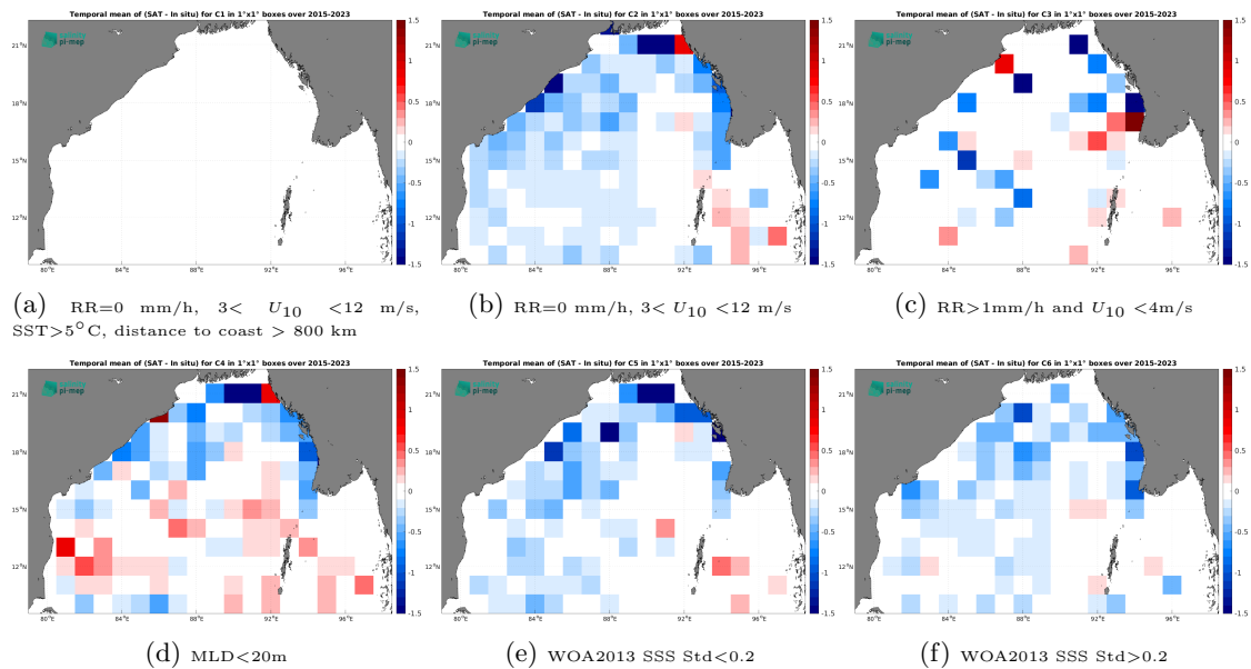
Figure 14: Temporal mean gridded over spatial boxes of size 1^\circ \times 1^\circ of \Delta SSS (SMAP SSS L3 v5.3 - Monthly (RSS) - Argo) for 6 different subdatasets corresponding to:RR=0 mm/h, 3 < U_{10} < 12 m/s, SST > 5^\circ\text{C} , distance to coast > 800 km (a), RR=0 mm/h, 3 < U_{10} < 12 m/s (b), RR > 1 mm/h and U_{10} < 4 m/s (c),MLD < 20 m (d),WOA2013 SSS Std < 0.2 (e),WOA2013 SSS Std > 0.2 (f).
