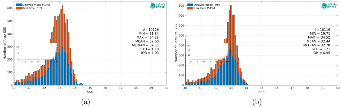
Figure 3: Histograms of SSS from Argo (a) and SMAP SSS L3 v5.3 - Monthly (RSS) (b) considering all match-up pairs per bins of 0.1 over the Bay of Bengal Pi-MEP region and for the full satellite product period.
