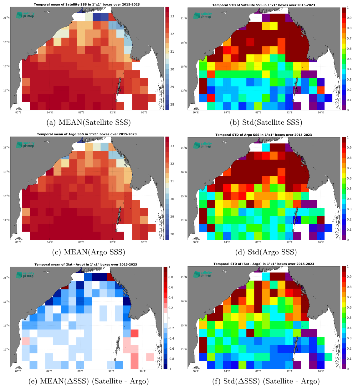
Figure 7: Temporal mean (left) and Std (right) of SSS from SMAP SSS L3 v5.3 - Monthly (RSS) (top), Argo (middle), and of \Delta SSS (Satellite - Argo). Only match-up pairs are used to generate these maps.
