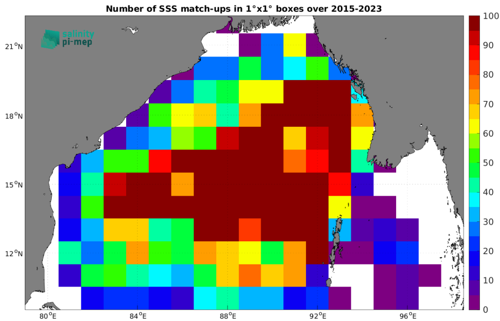
Figure 5: Number of SSS match-ups between Argo SSS and the SMAP SSS L3 v5.3 - Monthly (RSS) SSS product for the Bay of Bengal Pi-MEP region over 1^\circ \times 1^\circ boxes and for the full satellite product period.
