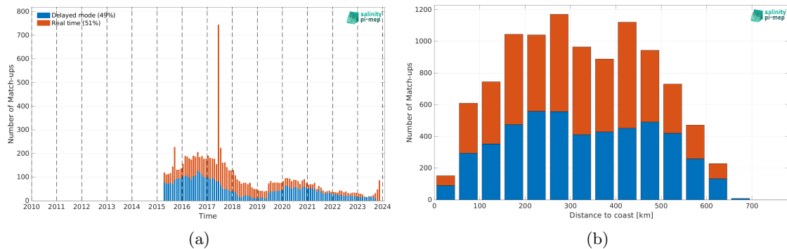
Figure 2: Number of match-ups between Argo and SMAP SSS L3 v5.3 - Monthly (RSS) SSS as a function of time (a) and as function of the distance to coast (b) over the Bay of Bengal Pi-MEP region and for the full satellite product period.
