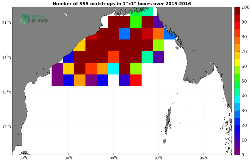
Figure 3: Number of SSS match-ups between Surface drifters SSS and the SMAP SSS L3 v5 - 8-Day running (RSS) SSS product for the Bay of Bengal Pi-MEP region over 1^\circ \times 1^\circ boxes and for the full satellite product period.
