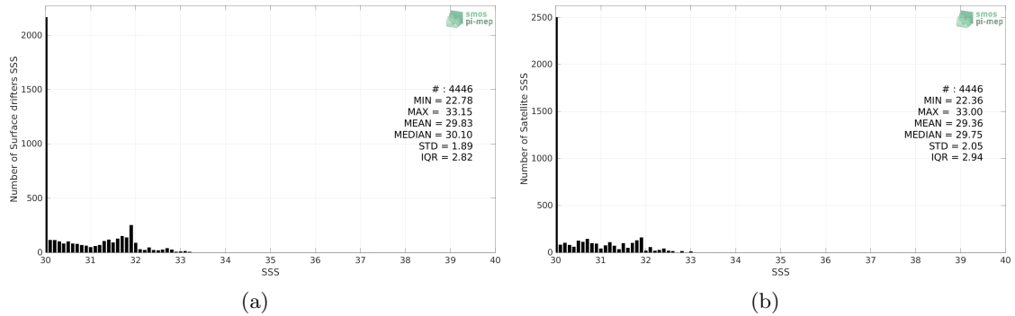
Figure 2: Histograms of SSS from Surface drifters (a) and SMAP SSS L3 v5 - 8-Day running (RSS) (b) considering all match-up pairs per bins of 0.1 over the Bay of Bengal Pi-MEP region and for the full satellite product period.
