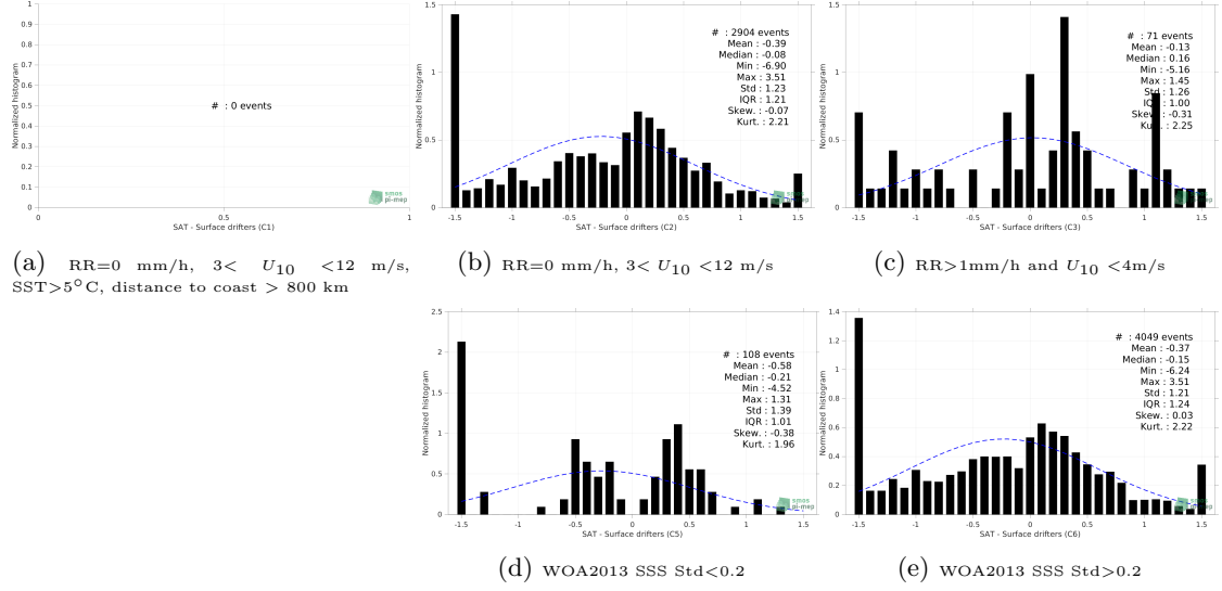
Figure 12: Normalized histogram of \Delta SSS (SMAP SSS L3 v5 - 8-Day running (RSS) - Surface drifters) for 5 different subdatasets corresponding to: RR=0 mm/h, 3 < U_{10} < 12 m/s, SST > 5°C, distance to coast > 800 km (a), RR=0 mm/h, 3 < U_{10} < 12 m/s (b), RR > 1mm/h and U_{10} < 4 m/s (c), WOA2013 SSS Std < 0.2 (d), WOA2013 SSS Std > 0.2 (e).
