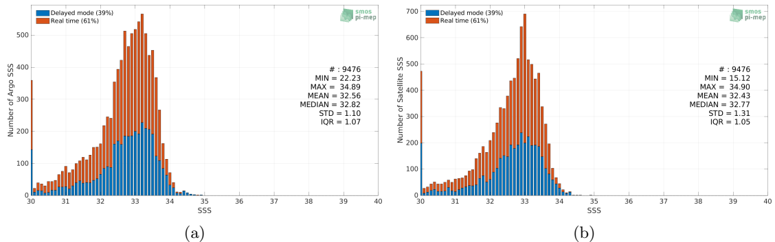
Figure 2: Histograms of SSS from Argo (a) and SMAP SSS L3 v5 - 8-Day running (RSS) (b) considering all match-up pairs per bins of 0.1 over the Bay of Bengal Pi-MEP region and for the full satellite product period.
