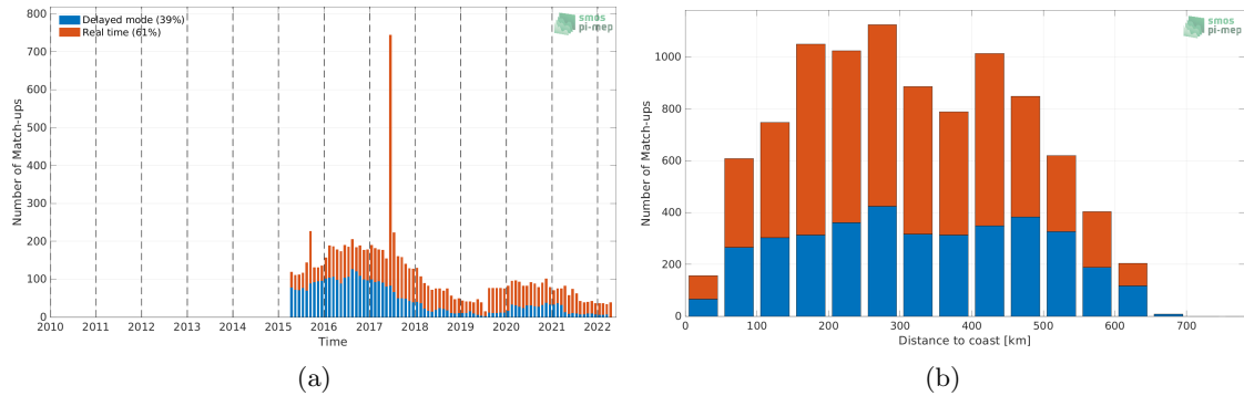
Figure 1: Number of match-ups between Argo and SMAP SSS L3 v5 - 8-Day running (RSS) SSS as a function of time (a) and as function of the distance to coast (b) over the Bay of Bengal Pi-MEP region and for the full satellite product period.
