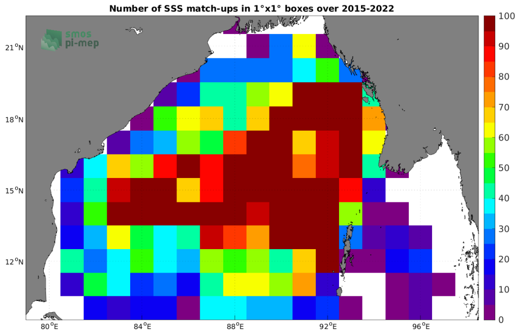
Figure 4: Number of SSS match-ups between Argo SSS and the SMAP SSS L3 v5 - 8-Day running (RSS) SSS product for the Bay of Bengal Pi-MEP region over 1^\circ \times 1^\circ boxes and for the full satellite product period.
