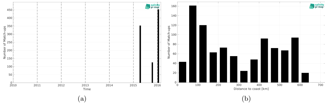
Figure 1: Number of match-ups between TSG (LEGOS-DM) and SMAP SSS L3 v5 - Monthly (RSS) SSS as a function of time (a) and as function of the distance to coast (b) over the Bay of Bengal Pi-MEP region and for the full satellite product period.
