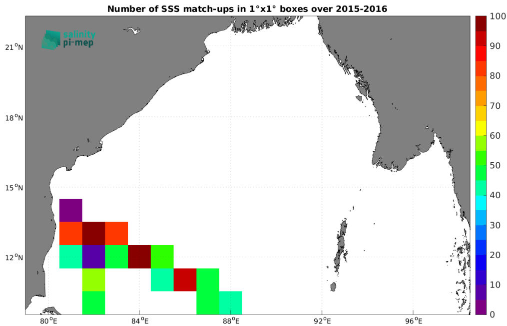
Figure 4: Number of SSS match-ups between TSG (LEGOS-DM) SSS and the SMAP SSS L3 v5 - Monthly (RSS) SSS product for the Bay of Bengal Pi-MEP region over 1^\circ \times 1^\circ boxes and for the full satellite product period.
