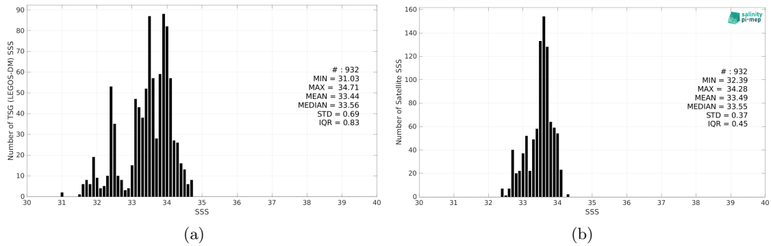
Figure 2: Histograms of SSS from TSG (LEGOS-DM) (a) and SMAP SSS L3 v5 - Monthly (RSS) (b) considering all match-up pairs per bins of 0.1 over the Bay of Bengal Pi-MEP region and for the full satellite product period.
