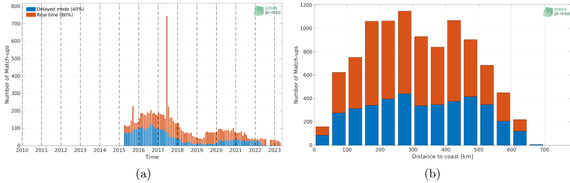
Figure 1: Number of match-ups between Argo and SMAP SSS L3 v5 - Monthly (RSS) SSS as a function of time (a) and as function of the distance to coast (b) over the Bay of Bengal Pi-MEP region and for the full satellite product period.
