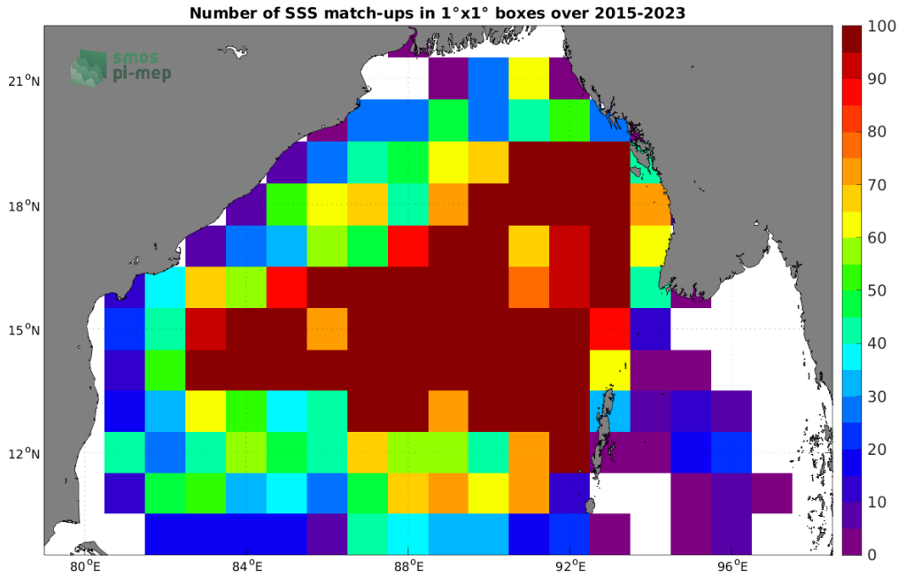
Figure 4: Number of SSS match-ups between Argo SSS and the SMAP SSS L3 v5 - Monthly (RSS) SSS product for the Bay of Bengal Pi-MEP region over 1^{\circ} \times 1^{\circ} boxes and for the full satellite product period.
