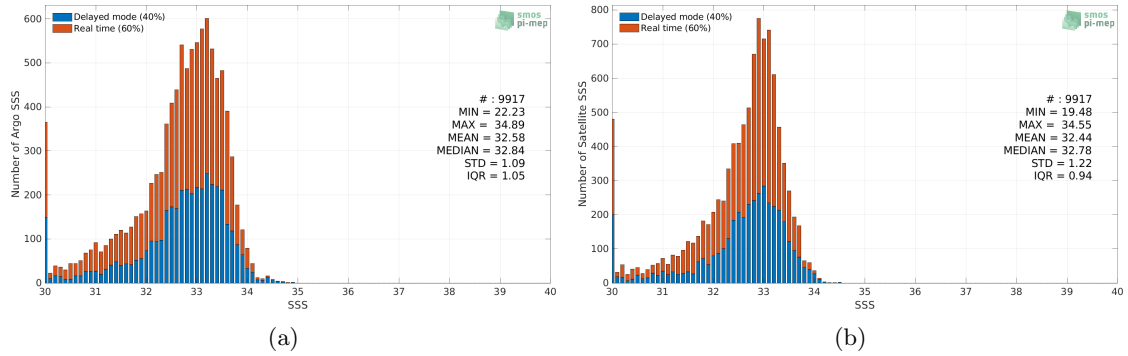
Figure 2: Histograms of SSS from Argo (a) and SMAP SSS L3 v5 - Monthly (RSS) (b) considering all match-up pairs per bins of 0.1 over the Bay of Bengal Pi-MEP region and for the full satellite product period.
