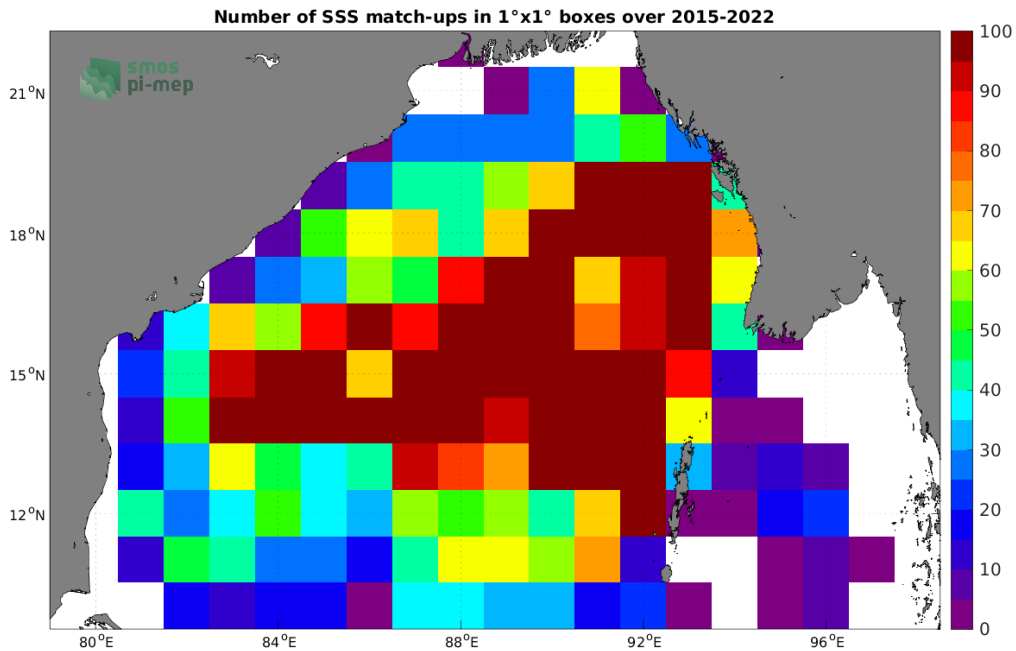
Figure 4: Number of SSS match-ups between Argo SSS and the SMAP SSS L3 v5 - Monthly (RSS) SSS product for the Bay of Bengal Pi-MEP region over 1^\circ \times 1^\circ boxes and for the full satellite product period.
