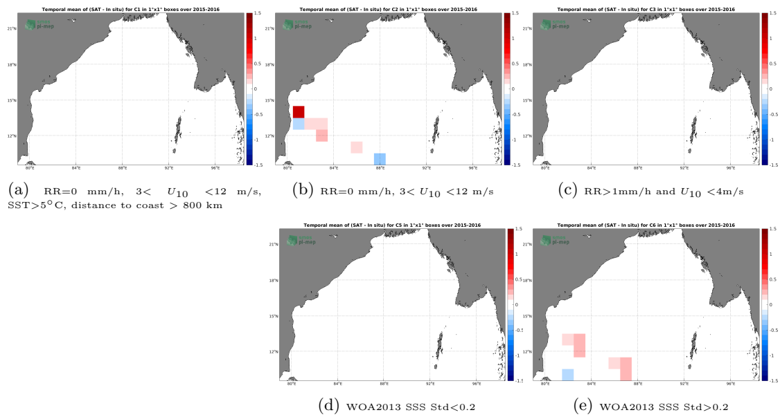
Figure 12: Temporal mean gridded over spatial boxes of size 1^\circ \times 1^\circ of \Delta SSS (SMAP SSS L3 v4 - 8-Day running (RSS) - TSG (LEGOS-DM)) for 5 different subdatasets corresponding to: RR=0 mm/h, 3 < U_{10} < 12 m/s, SST > 5^\circ C , distance to coast > 800 km (a), RR=0 mm/h, 3 < U_{10} < 12 m/s (b), RR > 1 mm/h and U_{10} < 4 m/s (c), WOA2013 SSS Std < 0.2 (d), WOA2013 SSS Std > 0.2 (e).
