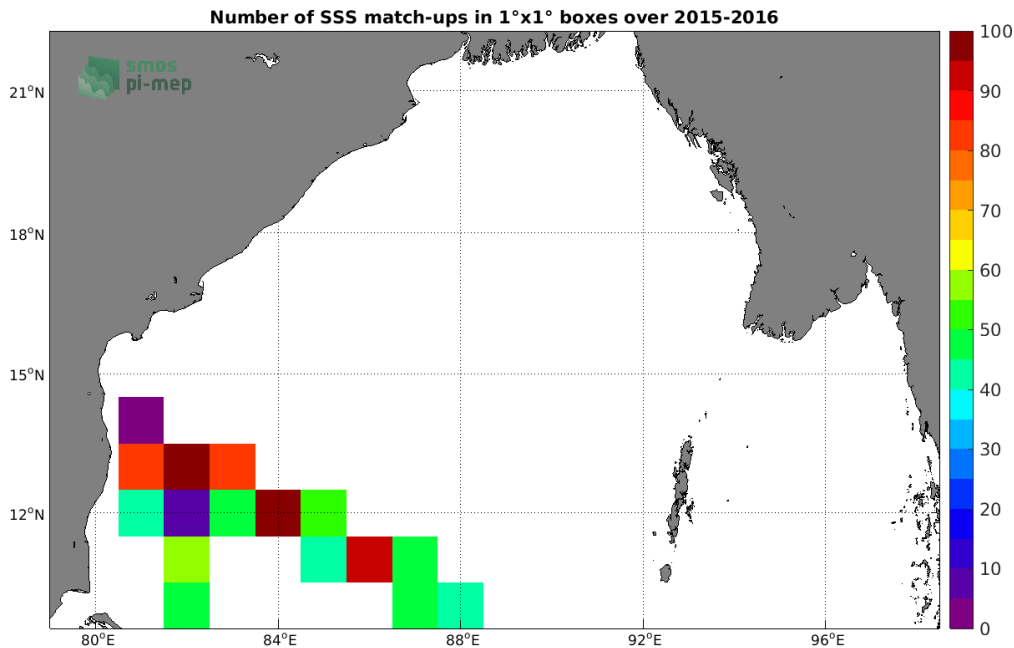
Figure 4: Number of SSS match-ups between TSG (LEGOS-DM) SSS and the SMAP SSS L3 v4 - 8-Day running (RSS) SSS product for the Bay of Bengal Pi-MEP region over 1°x1° boxes and for the full satellite product period.
