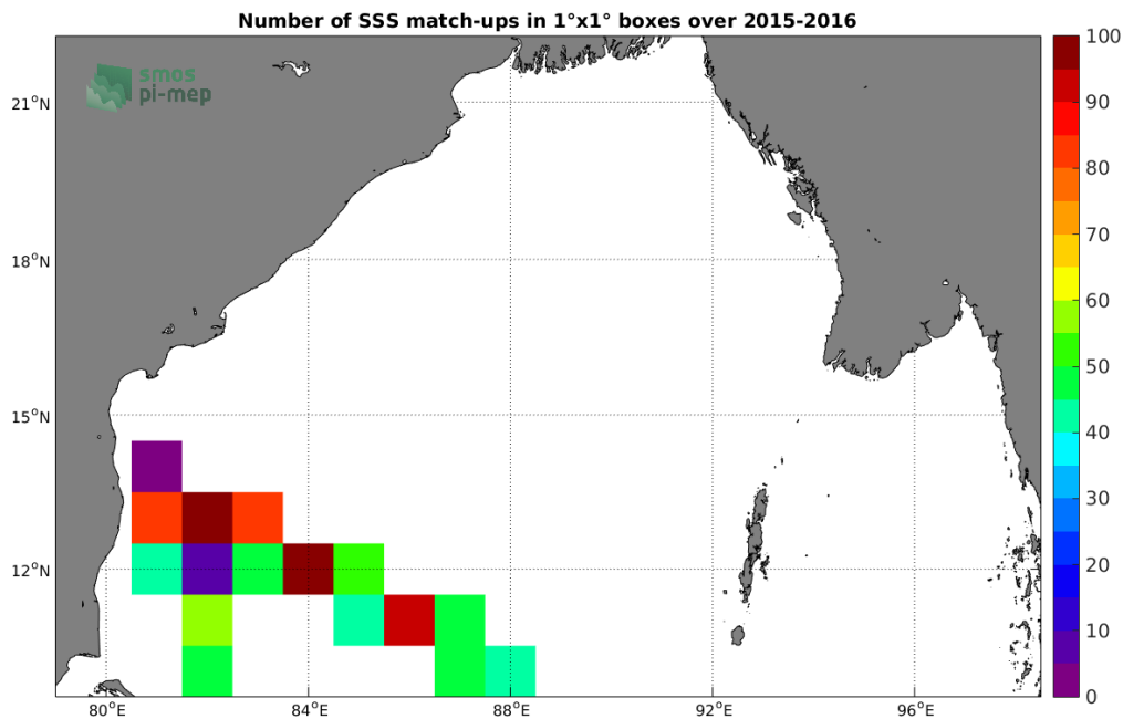
Figure 4: Number of SSS match-ups between TSG-LEGOS-DM SSS and the SMAP-L3-RSS-V4-8DAY-RUNNING SSS product for the Bay of Bengal Pi-MEP region over 1°x1° boxes and for the full satellite product period.
