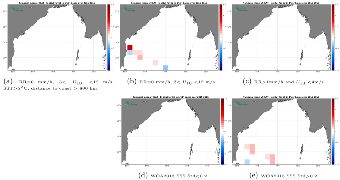
Figure 12: Temporal mean gridded over spatial boxes of size 1^\circ \times 1^\circ of \Delta SSS (SMAP-L3-RSS-V4-8DAY-RUNNING - TSG-LEGOS-DM) for 5 different subdatasets corresponding to:RR=0 mm/h, 3 < U_{10} < 12 m/s, SST > 5^\circ\text{C} , distance to coast > 800 km (a), RR=0 mm/h, 3 < U_{10} < 12 m/s (b), RR > 1 mm/h and U_{10} < 4 m/s (c), WOA2013 SSS Std < 0.2 (d), WOA2013 SSS Std > 0.2 (e).
