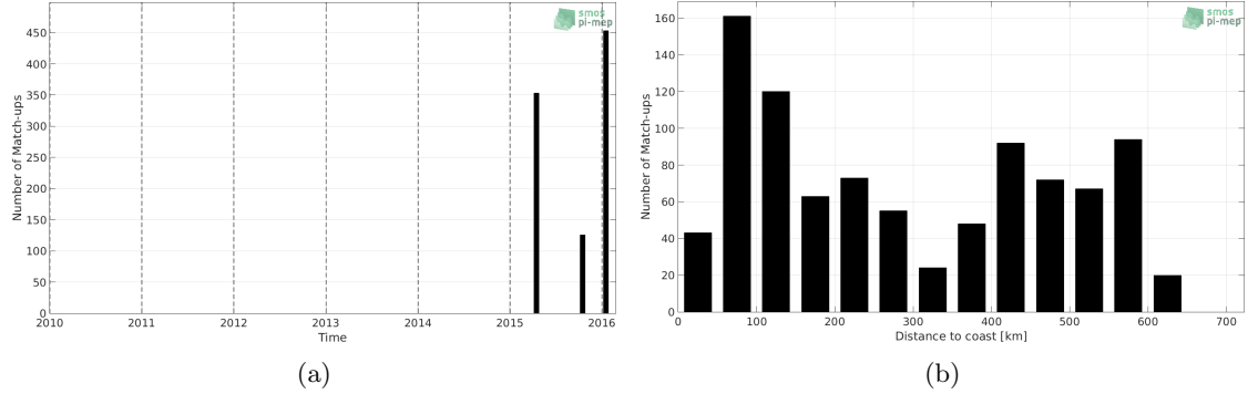
Figure 1: Number of match-ups between TSG-LEGOS-DM and SMAP-L3-RSS-V4-8DAY-RUNNING SSS as a function of time (a) and as function of the distance to coast (b) over the Bay of Bengal Pi-MEP region and for the full satellite product period.
