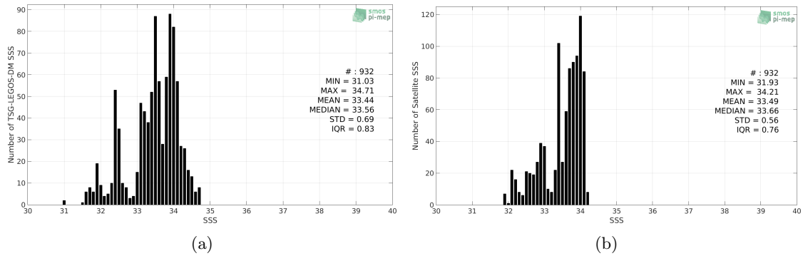
Figure 2: Histograms of SSS from TSG-LEGOS-DM (a) and SMAP-L3-RSS-V4-8DAY-RUNNING (b) considering all match-up pairs per bins of 0.1 over the Bay of Bengal Pi-MEP region and for the full satellite product period.
