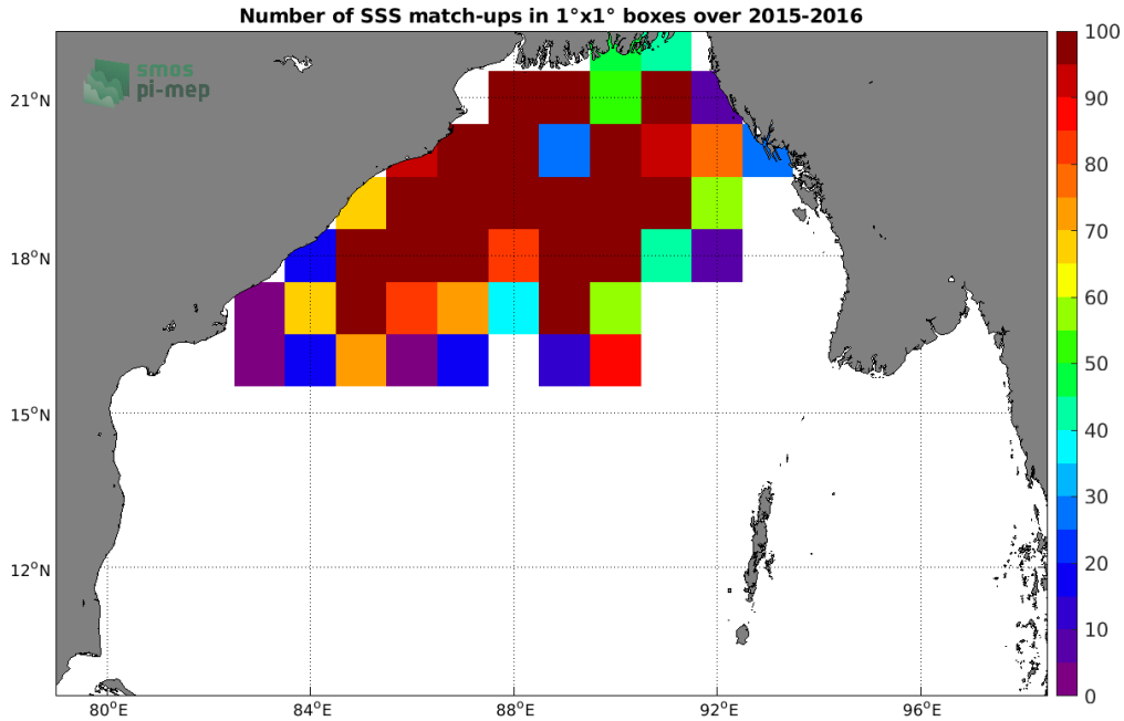
Figure 3: Number of SSS match-ups between Surface drifters SSS and the SMAP SSS L3 v4 - 8-Day running (RSS) SSS product for the Bay of Bengal Pi-MEP region over 1^\circ \times 1^\circ boxes and for the full satellite product period.
