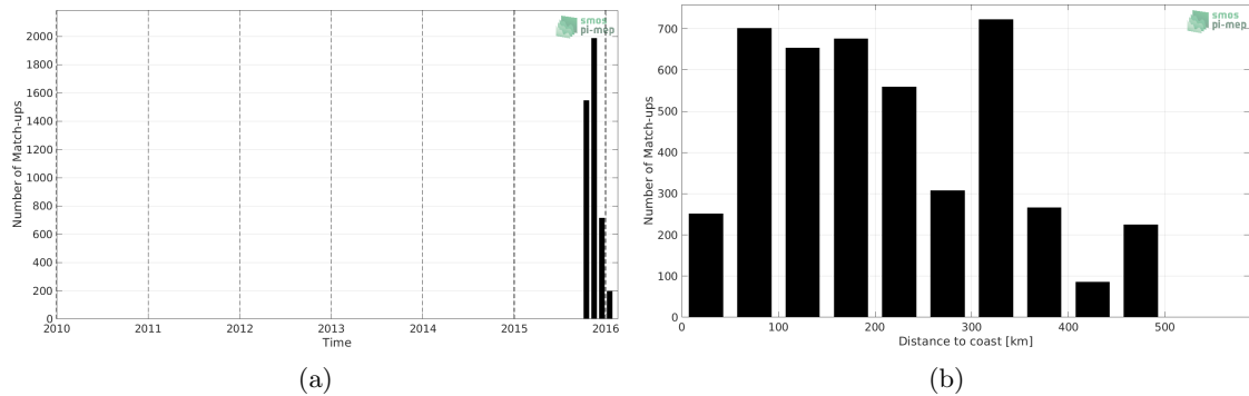
Figure 1: Number of match-ups between Surface drifters and SMAP SSS L3 v4 - 8-Day running (RSS) SSS as a function of time (a) and as function of the distance to coast (b) over the Bay of Bengal Pi-MEP region and for the full satellite product period.
