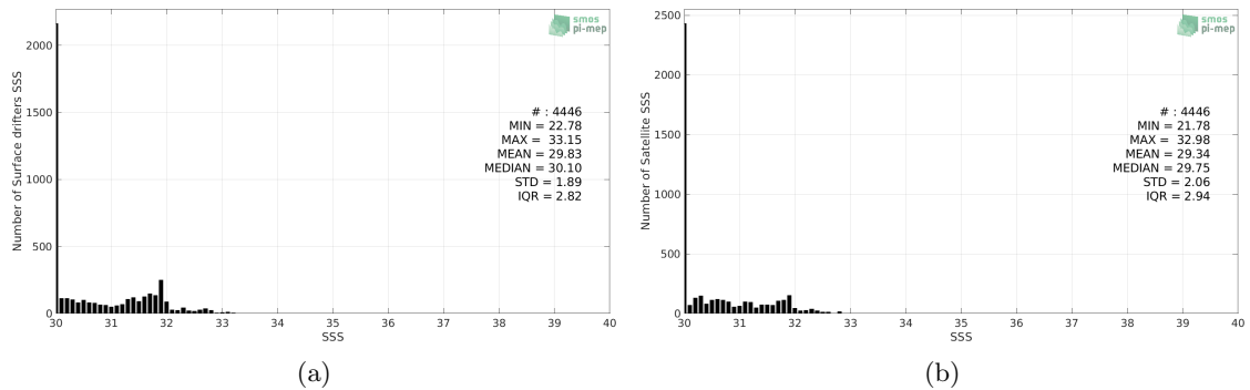
Figure 2: Histograms of SSS from Surface drifters (a) and SMAP SSS L3 v4 - 8-Day running (RSS) (b) considering all match-up pairs per bins of 0.1 over the Bay of Bengal Pi-MEP region and for the full satellite product period.
