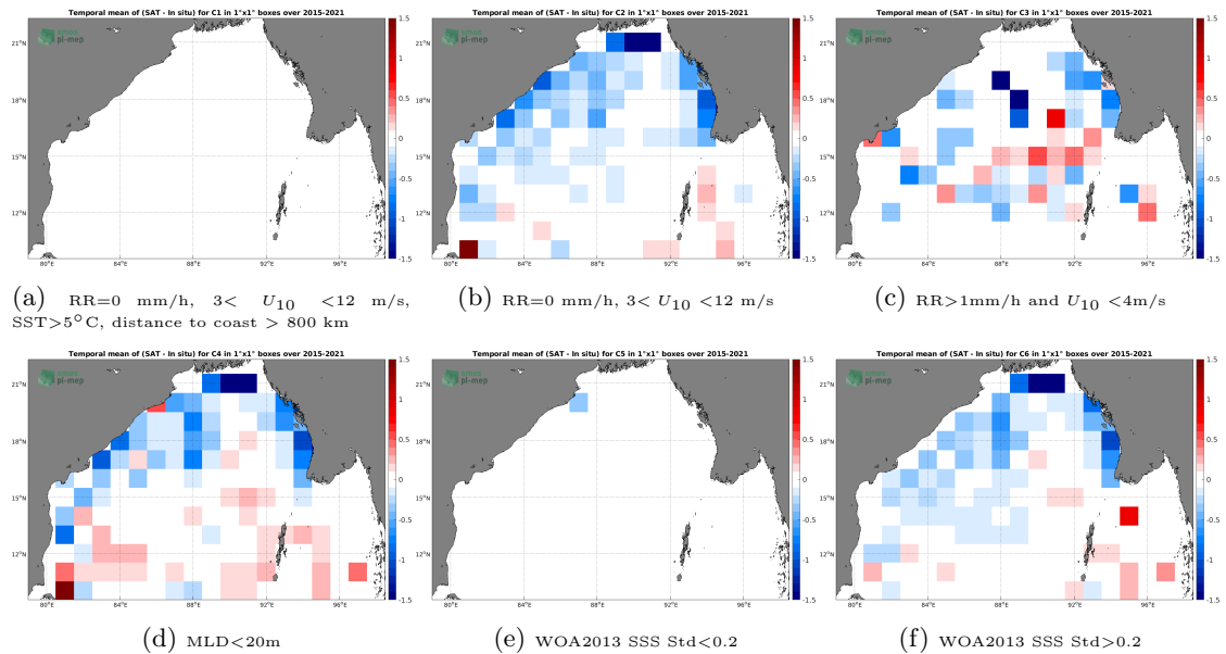
Figure 12: Temporal mean gridded over spatial boxes of size 1°x1° of \Delta SSS (SMAP SSS L3 v4 - 8-Day running (RSS) - Argo) for 6 different subdatasets corresponding to:RR=0 mm/h, 3 < U_{10} < 12 m/s, SST > 5°C, distance to coast > 800 km (a), RR=0 mm/h, 3 < U_{10} < 12 m/s (b), RR > 1mm/h and U_{10} < 4 m/s (c),MLD < 20m (d),WOA2013 SSS Std < 0.2 (e),WOA2013 SSS Std > 0.2 (f).
