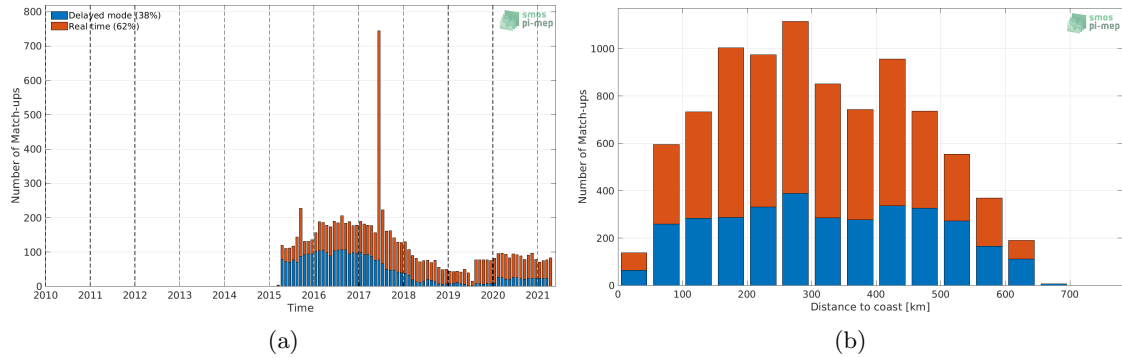
Figure 1: Number of match-ups between Argo and SMAP SSS L3 v4 - 8-Day running (RSS) SSS as a function of time (a) and as function of the distance to coast (b) over the Bay of Bengal Pi-MEP region and for the full satellite product period.
