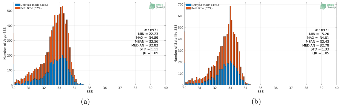
Figure 2: Histograms of SSS from Argo (a) and SMAP SSS L3 v4 - 8-Day running (RSS) (b) considering all match-up pairs per bins of 0.1 over the Bay of Bengal Pi-MEP region and for the full satellite product period.
