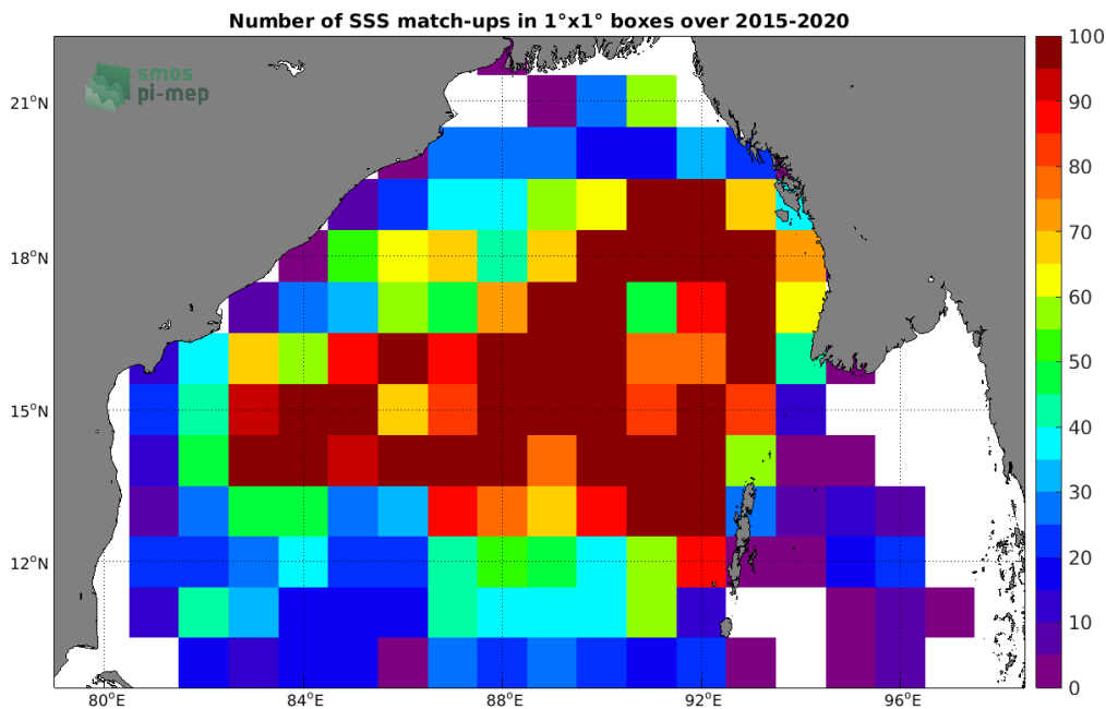
Figure 4: Number of SSS match-ups between Argo SSS and the SMAP SSS L3 v4 - 8-Day running (RSS) SSS product for the Bay of Bengal Pi-MEP region over 1°x1° boxes and for the full satellite product period.
