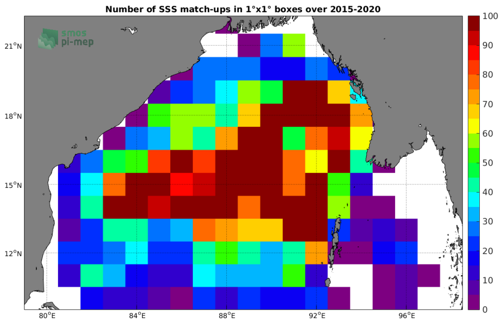
Figure 4: Number of SSS match-ups between Argo SSS and the SMAP-L3-RSS-V4-8DAY-RUNNING SSS product for the Bay of Bengal Pi-MEP region over 1°x1° boxes and for the full satellite product period.
