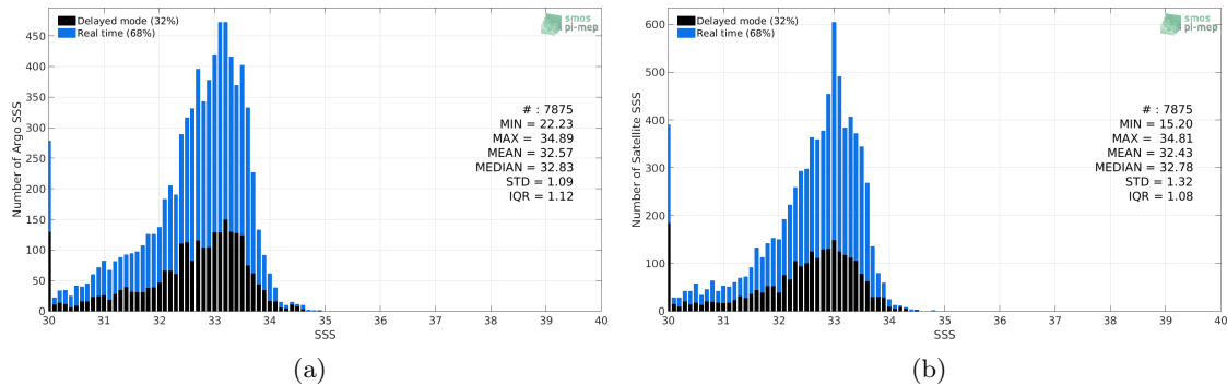
Figure 2: Histograms of SSS from Argo (a) and SMAP-L3-RSS-V4-8DAY-RUNNING (b) considering all match-up pairs per bins of 0.1 over the Bay of Bengal Pi-MEP region and for the full satellite product period.
