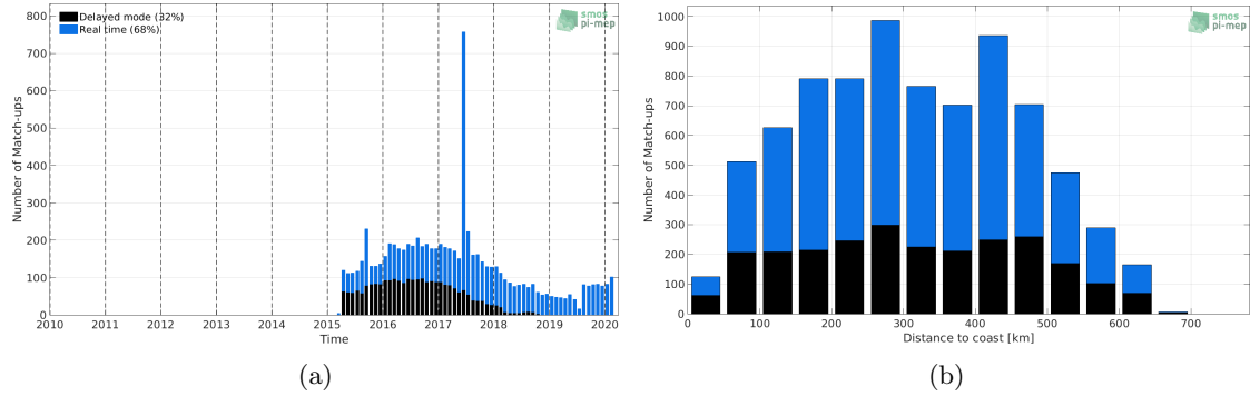
Figure 1: Number of match-ups between Argo and SMAP-L3-RSS-V4-8DAY-RUNNING SSS as a function of time (a) and as function of the distance to coast (b) over the Bay of Bengal Pi-MEP region and for the full satellite product period.
