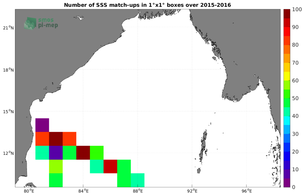
Figure 4: Number of SSS match-ups between TSG (LEGOS-DM) SSS and the SMAP SSS L3 v4 - Monthly (RSS) SSS product for the Bay of Bengal Pi-MEP region over 1^\circ \times 1^\circ boxes and for the full satellite product period.
