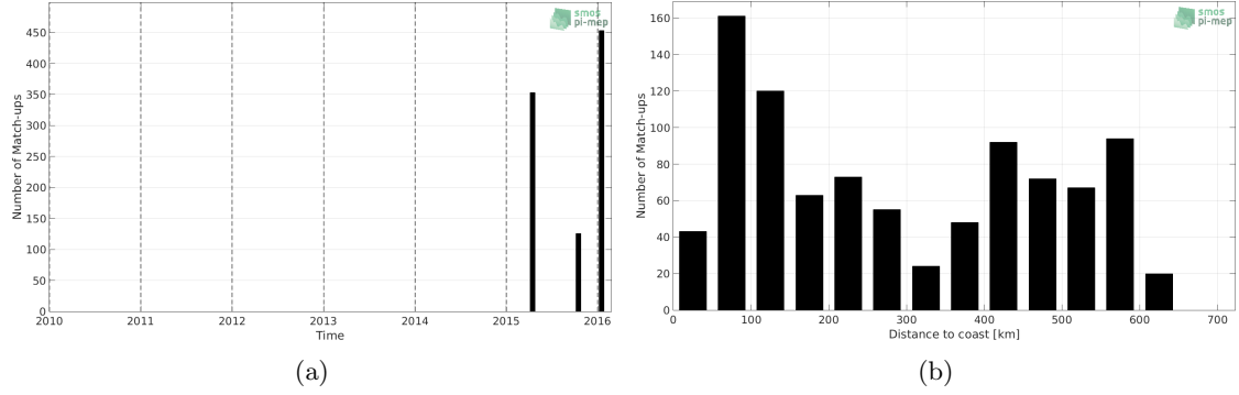
Figure 1: Number of match-ups between TSG-LEGOS-DM and SMAP-L3-RSS-V4-MONTHLY SSS as a function of time (a) and as function of the distance to coast (b) over the Bay of Bengal Pi-MEP region and for the full satellite product period.
