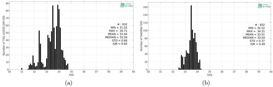
Figure 2: Histograms of SSS from TSG-LEGOS-DM (a) and SMAP-L3-RSS-V4-MONTHLY (b) considering all match-up pairs per bins of 0.1 over the Bay of Bengal Pi-MEP region and for the full satellite product period.
