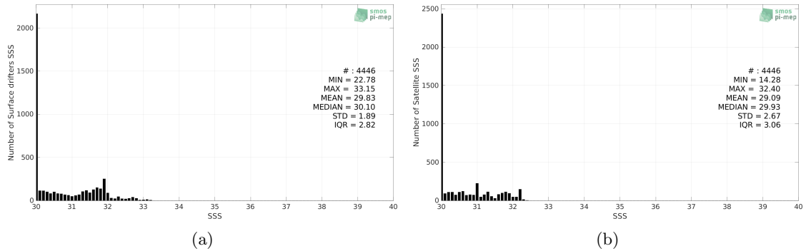
Figure 2: Histograms of SSS from Surface drifters (a) and SMAP SSS L3 v4 - Monthly (RSS) (b) considering all match-up pairs per bins of 0.1 over the Bay of Bengal Pi-MEP region and for the full satellite product period.
