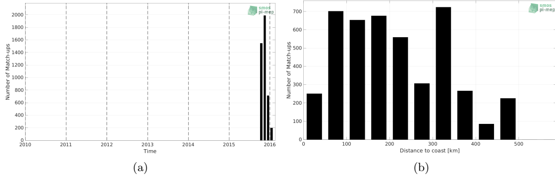
Figure 1: Number of match-ups between Surface drifters and SMAP SSS L3 v4 - Monthly (RSS) SSS as a function of time (a) and as function of the distance to coast (b) over the Bay of Bengal Pi-MEP region and for the full satellite product period.
