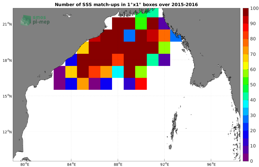
Figure 3: Number of SSS match-ups between Surface drifters SSS and the SMAP SSS L3 v4 - Monthly (RSS) SSS product for the Bay of Bengal Pi-MEP region over 1^\circ \times 1^\circ boxes and for the full satellite product period.
