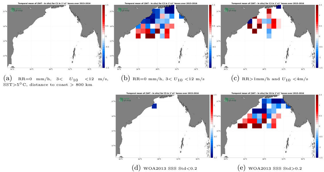
Figure 11: Temporal mean gridded over spatial boxes of size 1^\circ \times 1^\circ of \Delta SSS (SMAP SSS L3 v4 - Monthly (RSS) - Surface drifters) for 5 different subdatasets corresponding to:RR=0 mm/h, 3 < U_{10} < 12 m/s, SST >5^\circ\text{C} , distance to coast > 800 km (a), RR=0 mm/h, 3 < U_{10} < 12 m/s (b), RR >1 mm/h and U_{10} < 4 m/s (c), WOA2013 SSS Std <0.2 (d), WOA2013 SSS Std >0.2 (e).
