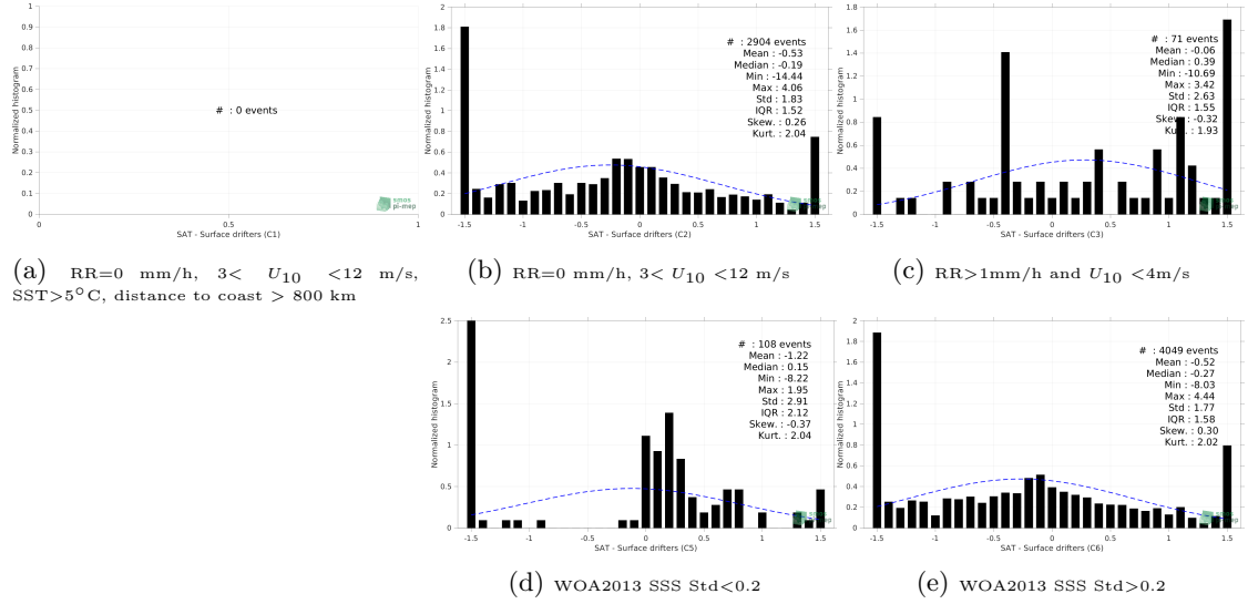
Figure 12: Normalized histogram of \Delta SSS (SMAP SSS L3 v4 - Monthly (RSS) - Surface drifters) for 5 different subdatasets corresponding to: RR=0 mm/h, 3 < U_{10} < 12 m/s, SST > 5°C, distance to coast > 800 km (a), RR=0 mm/h, 3 < U_{10} < 12 m/s (b), RR > 1mm/h and U_{10} < 4 m/s (c), WOA2013 SSS Std < 0.2 (d), WOA2013 SSS Std > 0.2 (e).
