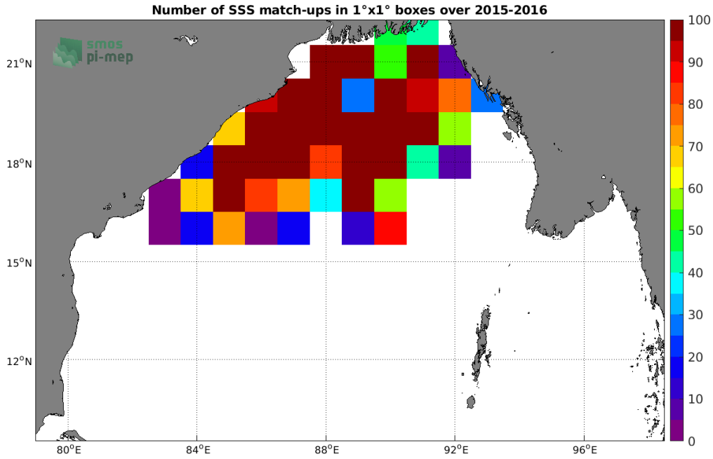
Figure 3: Number of SSS match-ups between Surface drifters SSS and the SMAP SSS L3 v4 - Monthly (RSS) SSS product for the Bay of Bengal Pi-MEP region over 1^{\circ} \times 1^{\circ} boxes and for the full satellite product period.
