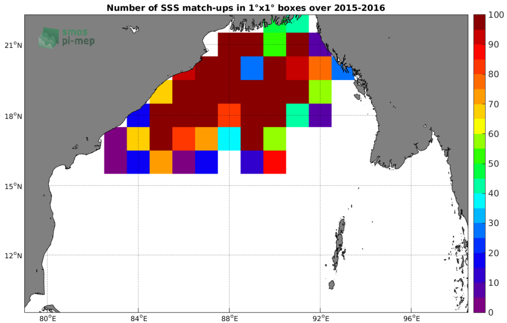
Figure 3: Number of SSS match-ups between Surface drifters SSS and the SMAP-L3-RSS-V4-MONTHLY SSS product for the Bay of Bengal Pi-MEP region over 1^\circ \times 1^\circ boxes and for the full satellite product period.
