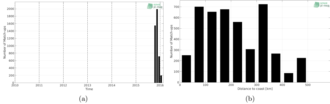
Figure 1: Number of match-ups between Surface drifters and SMAP-L3-RSS-V4-MONTHLY SSS as a function of time (a) and as function of the distance to coast (b) over the Bay of Bengal Pi-MEP region and for the full satellite product period.
