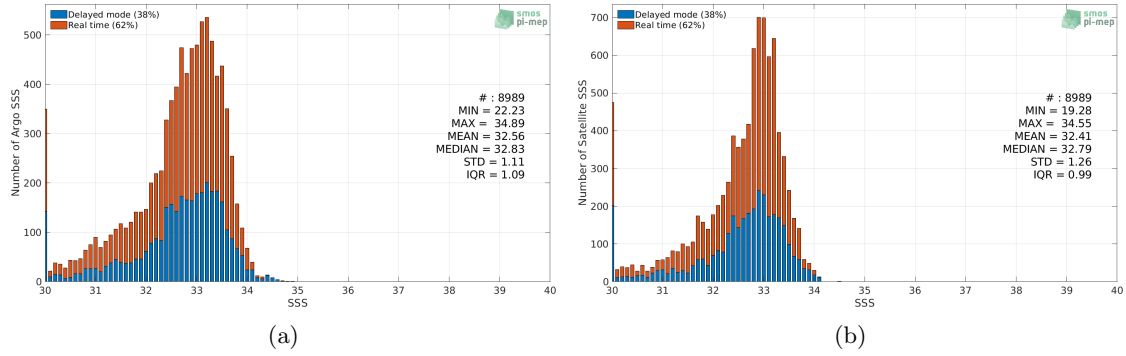
Figure 2: Histograms of SSS from Argo (a) and SMAP SSS L3 v4 - Monthly (RSS) (b) considering all match-up pairs per bins of 0.1 over the Bay of Bengal Pi-MEP region and for the full satellite product period.
