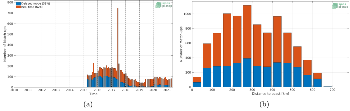
Figure 1: Number of match-ups between Argo and SMAP SSS L3 v4 - Monthly (RSS) SSS as a function of time (a) and as function of the distance to coast (b) over the Bay of Bengal Pi-MEP region and for the full satellite product period.
