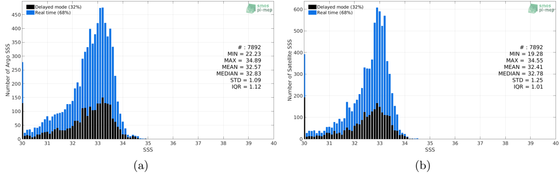
Figure 2: Histograms of SSS from Argo (a) and SMAP-L3-RSS-V4-MONTHLY (b) considering all match-up pairs per bins of 0.1 over the Bay of Bengal Pi-MEP region and for the full satellite product period.
