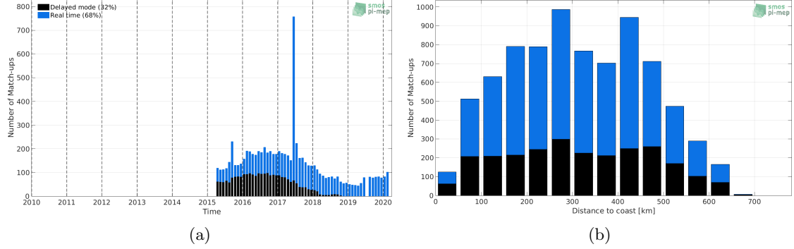
Figure 1: Number of match-ups between Argo and SMAP-L3-RSS-V4-MONTHLY SSS as a function of time (a) and as function of the distance to coast (b) over the Bay of Bengal Pi-MEP region and for the full satellite product period.
