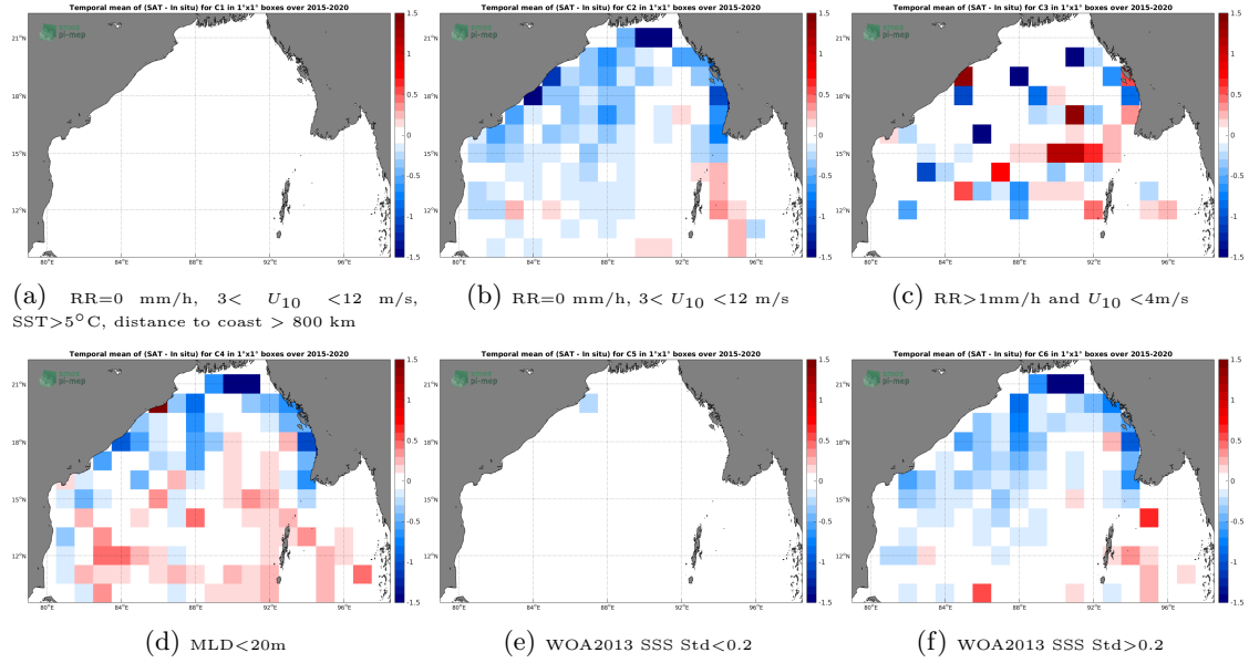
Figure 12: Temporal mean gridded over spatial boxes of size 1^\circ \times 1^\circ of \Delta SSS (SMAP-L3-RSS-V4-MONTHLY - Argo) for 6 different subdatasets corresponding to:RR=0 mm/h, 3 < U_{10} < 12 m/s, SST >5^\circ C, distance to coast > 800 km (a), RR=0 mm/h, 3 < U_{10} < 12 m/s (b), RR >1 mm/h and U_{10} < 4 m/s (c),MLD <20 m (d),WOA2013 SSS Std <0.2 (e),WOA2013 SSS Std >0.2 (f).
