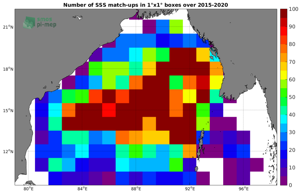
Figure 4: Number of SSS match-ups between Argo SSS and the SMAP-L3-RSS-V4-MONTHLY SSS product for the Bay of Bengal Pi-MEP region over 1^\circ \times 1^\circ boxes and for the full satellite product period.
