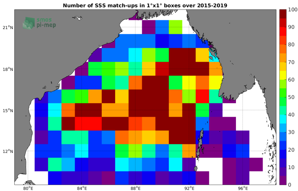
Figure 4: Number of SSS match-ups between Argos SSS and the SMAP-L3-RSS-V4-MONTHLY SSS product for the Bay of Bengal Pi-MEP region over 1^{\circ} \times 1^{\circ} boxes and for the full satellite product period.
