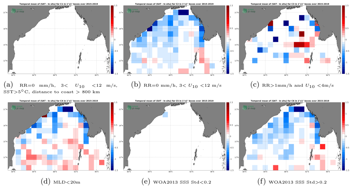
Figure 12: Temporal mean gridded over spatial boxes of size 1^\circ \times 1^\circ of \Delta SSS (SMAP-L3-RSS-V4-MONTHLY - Argo) for 6 different subsets corresponding to:RR=0 mm/h, 3 < U_{10} < 12 m/s, SST >5^\circ\text{C} , distance to coast > 800 km (a), RR=0 mm/h, 3 < U_{10} < 12 m/s (b), RR >1 mm/h and U_{10} < 4 m/s (c),MLD <20 m (d),WOA2013 SSS Std <0.2 (e),WOA2013 SSS Std >0.2 (f).
