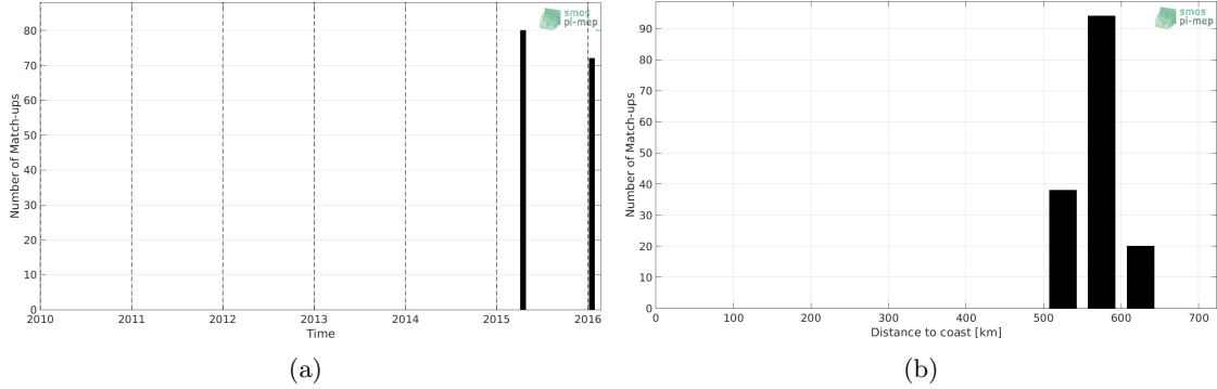
Figure 1: Number of match-ups between TSG-LEGOS-DM and SMAP-L3-RSS-V3-8DAY-RUNNING-70KM SSS as a function of time (a) and as function of the distance to coast (b) over the Bay of Bengal Pi-MEP region and for the full satellite product period.
