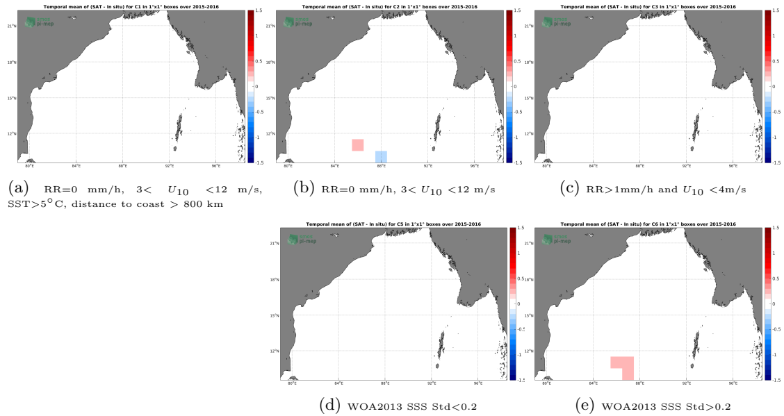
Figure 12: Temporal mean gridded over spatial boxes of size 1^\circ \times 1^\circ of \Delta SSS (SMAP-L3-RSS-V3-8DAY-RUNNING-70KM - TSG-LEGOS-DM) for 5 different subdatasets corresponding to:RR=0 mm/h, 3 < U_{10} < 12 m/s, SST >5^\circ C, distance to coast > 800 km (a), RR=0 mm/h, 3 < U_{10} < 12 m/s (b), RR >1 mm/h and U_{10} < 4 m/s (c), WOA2013 SSS Std <0.2 (d), WOA2013 SSS Std >0.2 (e).
