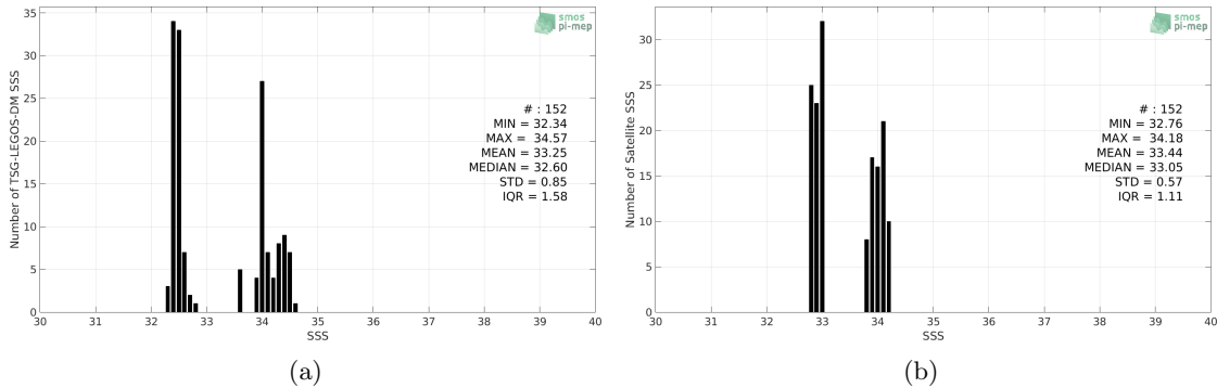
Figure 2: Histograms of SSS from TSG-LEGOS-DM (a) and SMAP-L3-RSS-V3-8DAY-RUNNING-70KM (b) considering all match-up pairs per bins of 0.1 over the Bay of Bengal Pi-MEP region and for the full satellite product period.
