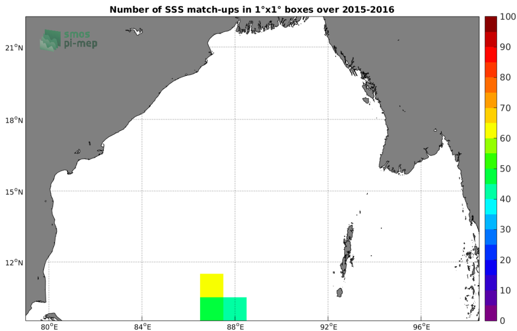
Figure 4: Number of SSS match-ups between TSG-LEGOS-DM SSS and the SMAP-L3-RSS-V3-8DAY-RUNNING-70KM SSS product for the Bay of Bengal Pi-MEP region over 1^\circ \times 1^\circ boxes and for the full satellite product period.
