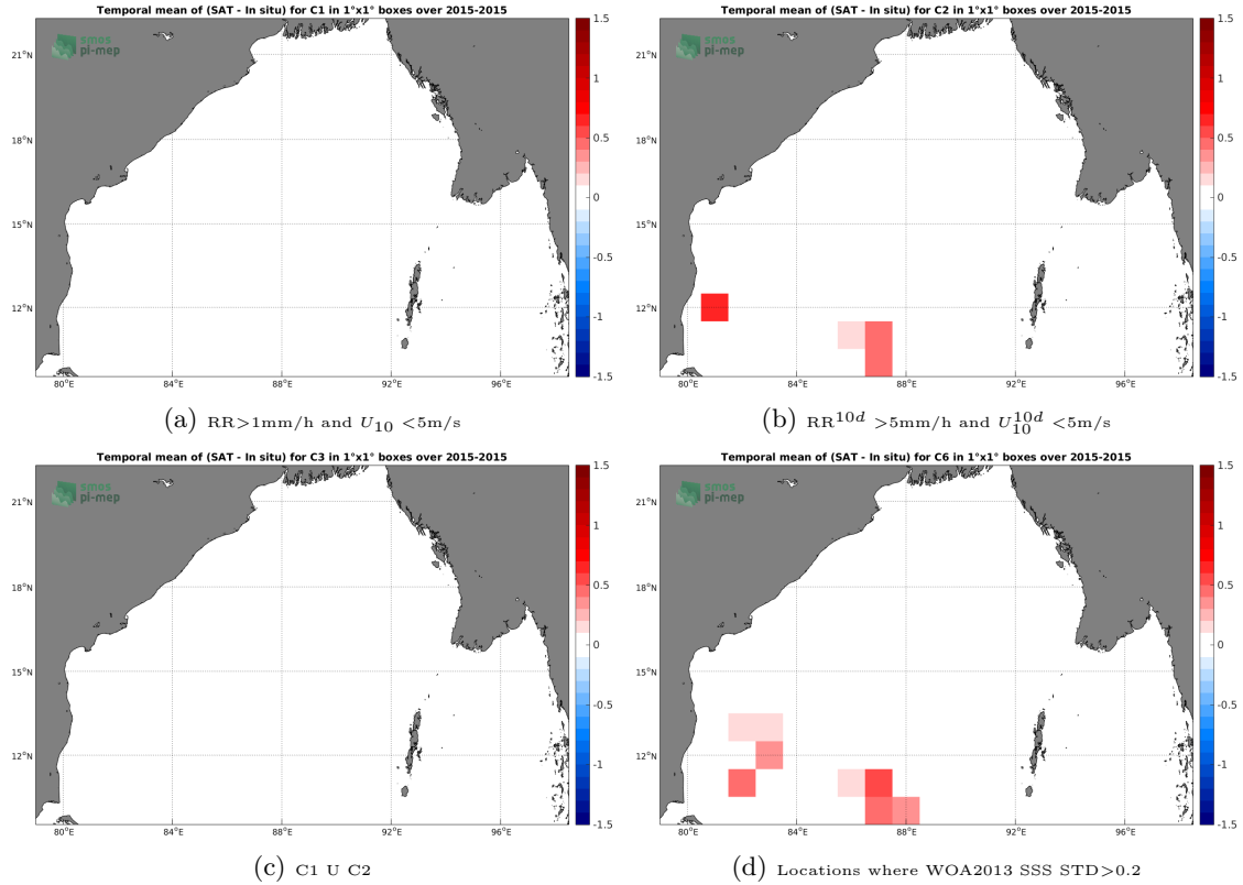
Figure 12: Temporal mean gridded over spatial boxes of size 1^\circ \times 1^\circ of \Delta SSS (SMAP-L3-RSS-V3-8DAY-RUNNING-70KM - TSG-LEGOS-DM) for 4 different subdatasets corresponding to: RR > 1mm/h and U_{10} < 5\text{m/s} (a), RR^{10d} > 5\text{mm/h} and U_{10}^{10d} < 5\text{m/s} (b), C1 U C2 (c), Locations where WOA2013 SSS STD > 0.2 (d).
