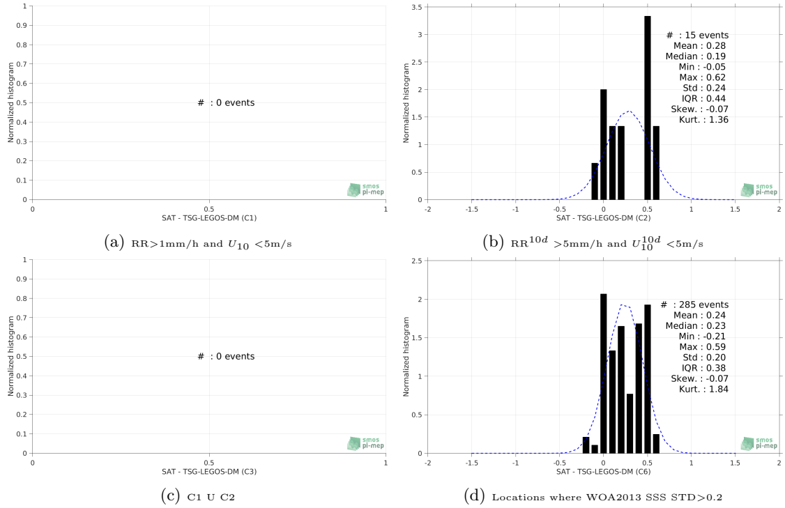
Figure 13: Normalized histogram of \Delta\text{SSS} (SMAP-L3-RSS-V3-8DAY-RUNNING-70KM - TSG-LEGOS-DM) for 6 different subdatasets corresponding to: RR > 1\text{mm/h} and U_{10} < 5\text{m/s} (a), RR^{10d} > 5\text{mm/h} and U_{10}^{10d} < 5\text{m/s} (b), C1 \cup C2 (c), Locations where WOA2013 SSS STD > 0.2 (d).
