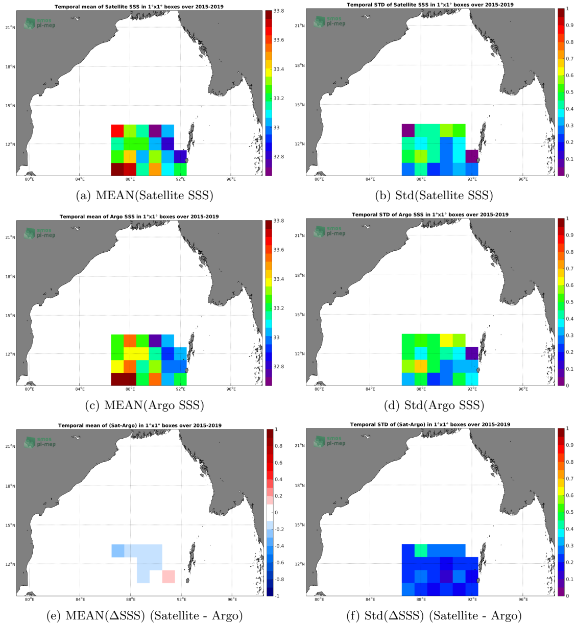
Figure 6: Temporal mean (left) and Std (right) of SSS from SMAP-L3-RSS-V3-8DAY-RUNNING-70KM (top), Argo in situ (middle), and of \Delta SSS (Satellite - Argo). Only match-up pairs are used to generate these maps.
