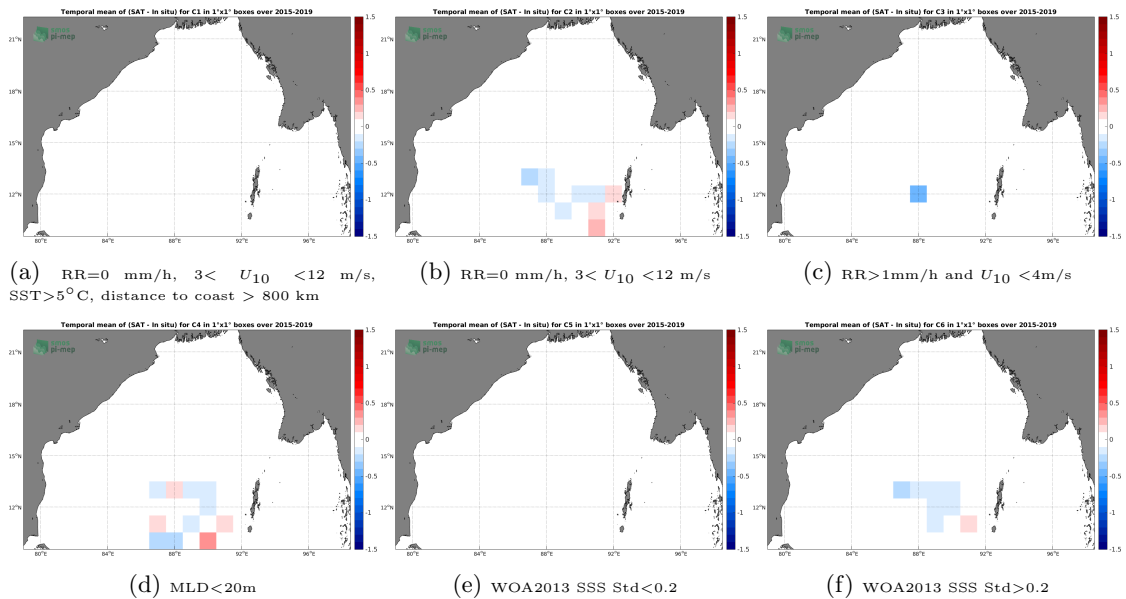
Figure 12: Temporal mean gridded over spatial boxes of size 1^\circ \times 1^\circ of \Delta SSS (SMAP-L3-RSS-V3-8DAY-RUNNING-70KM - Argo) for 6 different subdatasets corresponding to:RR=0 mm/h, 3 < U_{10} < 12 m/s, SST >5^\circ C, distance to coast > 800 km (a), RR=0 mm/h, 3 < U_{10} < 12 m/s (b), RR >1 mm/h and U_{10} < 4 m/s (c),MLD <20 m (d),WOA2013 SSS Std <0.2 (e),WOA2013 SSS Std >0.2 (f).
