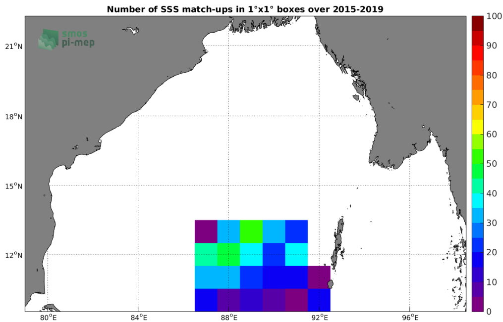
Figure 4: Number of SSS match-ups between Argo SSS and the SMAP-L3-RSS-V3-8DAY-RUNNING-70KM SSS product for the Bay of Bengal Pi-MEP region over 1^{\circ} \times 1^{\circ} boxes and for the full satellite product period.
