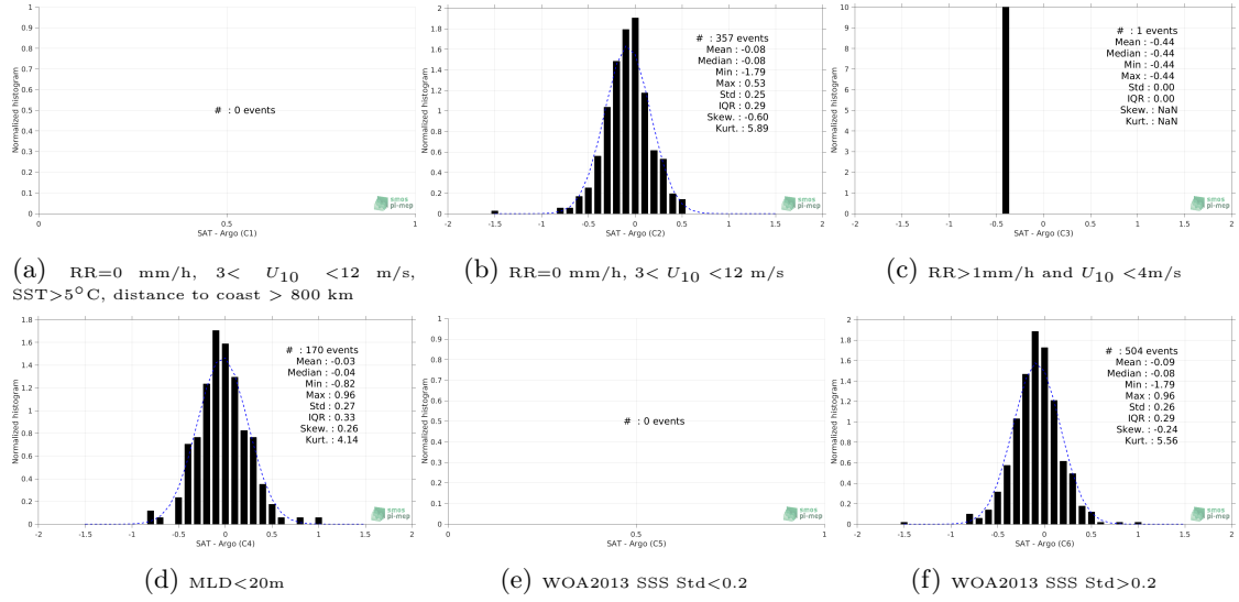
Figure 13: Normalized histogram of \Delta SSS (SMAP-L3-RSS-V3-8DAY-RUNNING-70KM - Argo) for 6 different subdatasets corresponding to: RR=0 mm/h, 3 < U_{10} < 12 m/s, SST>5°C, distance to coast > 800 km (a), RR=0 mm/h, 3 < U_{10} < 12 m/s (b), RR>1mm/h and U_{10} < 4 m/s (c), MLD<20m (d), WOA2013 SSS Std<0.2 (e), WOA2013 SSS Std>0.2 (f).
