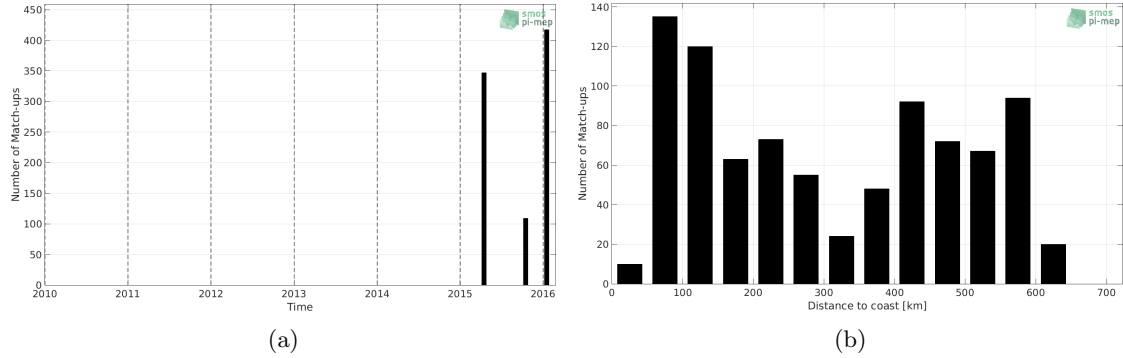
Figure 1: Number of match-ups between TSG-LEGOS-DM and SMAP-L3-RSS-V3-8DAY-RUNNING-40KM SSS as a function of time (a) and as function of the distance to coast (b) over the Bay of Bengal Pi-MEP region and for the full satellite product period.
