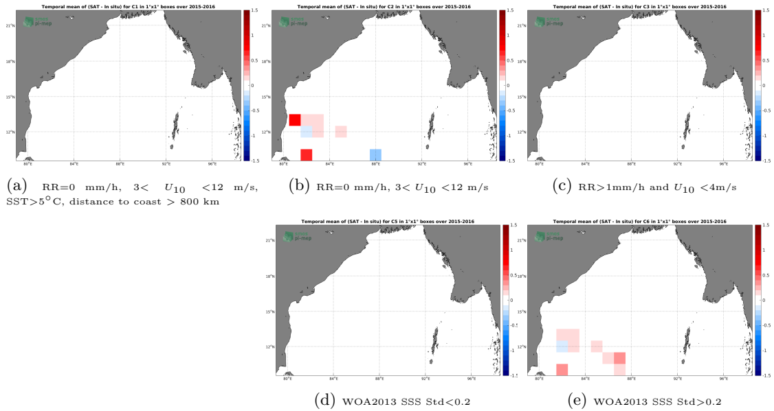
Figure 12: Temporal mean gridded over spatial boxes of size 1^\circ \times 1^\circ of \Delta SSS (SMAP-L3-RSS-V3-8DAY-RUNNING-40KM - TSG-LEGOS-DM) for 5 different subdatasets corresponding to:RR=0 mm/h, 3 < U_{10} < 12 m/s, SST >5^\circ C, distance to coast > 800 km (a), RR=0 mm/h, 3 < U_{10} < 12 m/s (b), RR >1 mm/h and U_{10} < 4 m/s (c), WOA2013 SSS Std <0.2 (d), WOA2013 SSS Std >0.2 (e).
