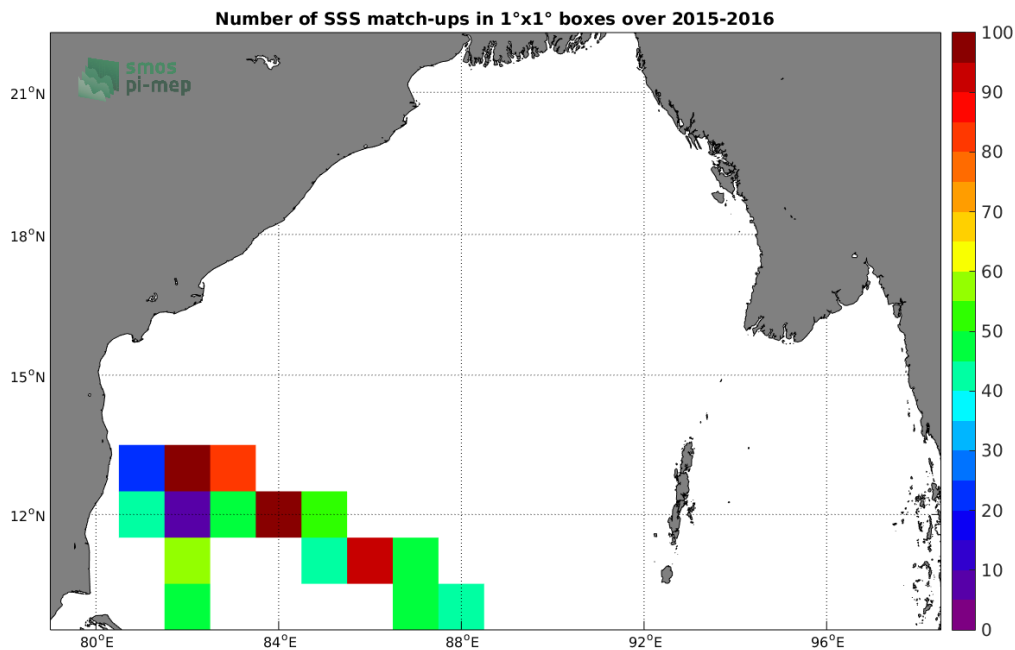
Figure 4: Number of SSS match-ups between TSG-LEGOS-DM SSS and the SMAP-L3-RSS-V3-8DAY-RUNNING-40KM SSS product for the Bay of Bengal Pi-MEP region over 1^{\circ} \times 1^{\circ} boxes and for the full satellite product period.
