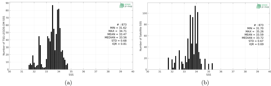
Figure 2: Histograms of SSS from TSG-LEGOS-DM (a) and SMAP-L3-RSS-V3-8DAY-RUNNING-40KM (b) considering all match-up pairs per bins of 0.1 over the Bay of Bengal Pi-MEP region and for the full satellite product period.
