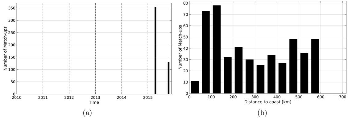
Figure 1: Number of match-ups between TSG-LEGOS-DM and SMAP-L3-RSS-V2-8DAY-RUNNING-40KM SSS as a function of time (a) and as function of the distance to coast (b) over the Bay of Bengal Pi-MEP region and for the full satellite product period.
