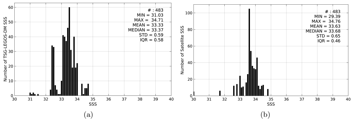
Figure 2: Histograms of SSS from TSG-LEGOS-DM (a) and SMAP-L3-RSS-V2-8DAY-RUNNING-40KM (b) considering all match-up pairs per bins of 0.1 over the Bay of Bengal Pi-MEP region and for the full satellite product period.
