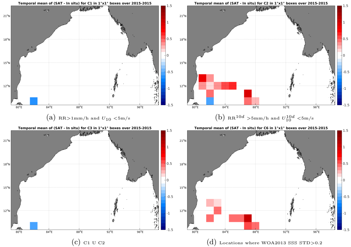
Figure 12: Temporal mean gridded over spatial boxes of size 1^\circ \times 1^\circ of \Delta SSS (SMAP-L3-RSS-V2-8DAY-RUNNING-40KM - TSG-LEGOS-DM) for 4 different subdatasets corresponding to:RR > 1mm/h and U_{10} < 5 m/s (a), RR^{10d} > 5 mm/h and U_{10}^{10d} < 5 m/s (b), C1 U C2 (c),Locations where WOA2013 SSS STD > 0.2 (d).
