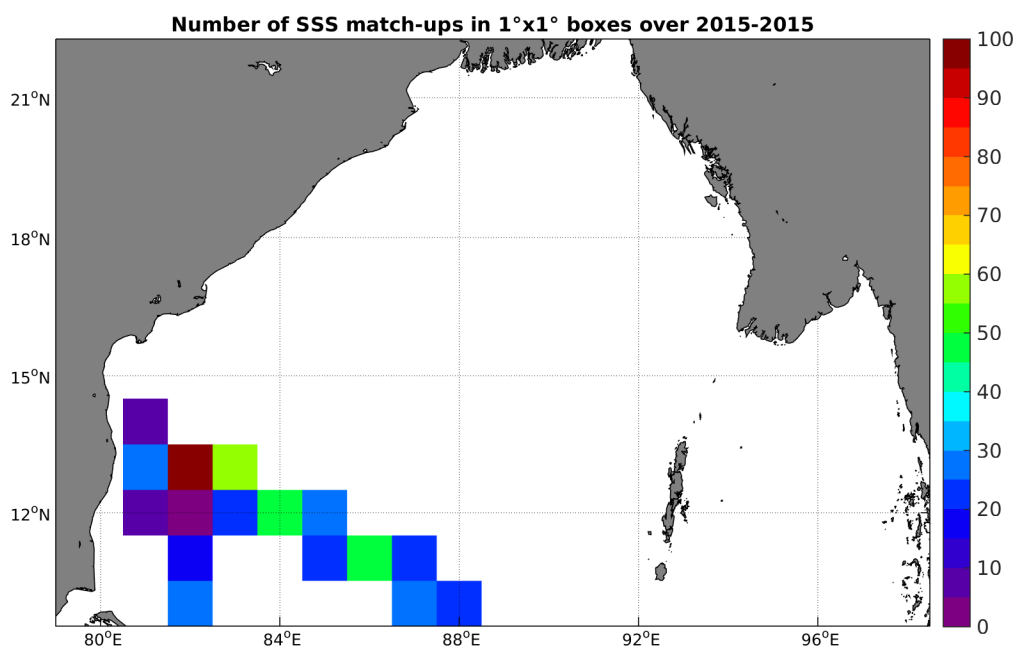
Figure 4: Number of SSS match-ups between TSG-LEGOS-DM SSS and the SMAP-L3-RSS-V2-8DAY-RUNNING-40KM SSS product for the Bay of Bengal Pi-MEP region over 1°x1° boxes and for the full satellite product period.
