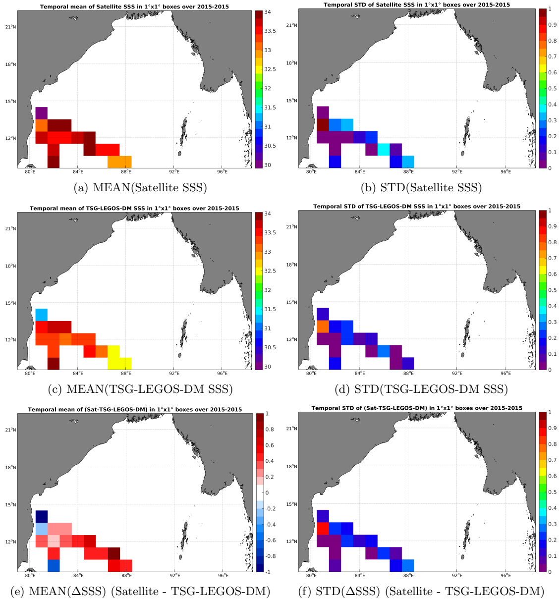
Figure 6: Temporal mean (left) and STD (right) of SSS from SMAP-L3-RSS-V2-8DAY-RUNNING-40KM (top), TSG-LEGOS-DM (middle), and of \Delta SSS (Satellite - TSG-LEGOS-DM). Only match-up pairs are used to generate these maps.
