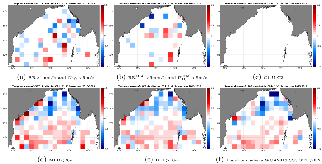
Figure 12: Temporal mean gridded over spatial boxes of size 1^\circ \times 1^\circ of \Delta SSS (SMAP-L3-RSS-V2-8DAY-RUNNING-40KM - Argo) for 6 different subdatasets corresponding to:RR>1mm/h and U_{10} < 5\text{m/s} (a), RR^{10d} > 5\text{mm/h} and U_{10}^{10d} < 5\text{m/s} (b), C1 U C2 (c),MLD<20m (d),BLT>10m (e),Locations where WOA2013 SSS STD>0.2 (f).
