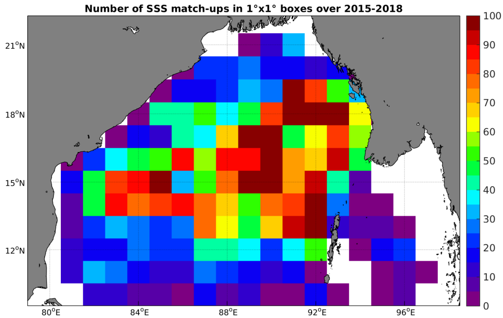
Figure 4: Number of SSS match-ups between Argo SSS and the SMAP-L3-RSS-V2-8DAY-RUNNING-40KM SSS product for the Bay of Bengal Pi-MEP region over 1°x1° boxes and for the full satellite product period.
