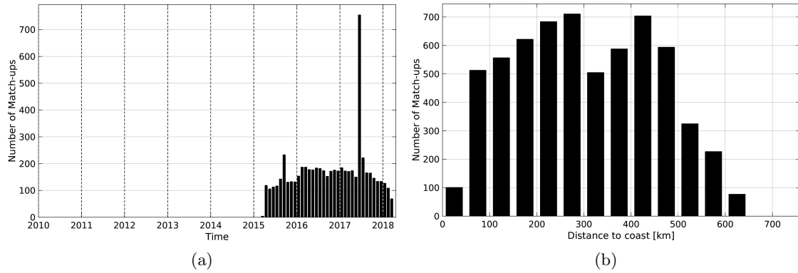
Figure 1: Number of match-ups between Argo and SMAP-L3-RSS-V2-8DAY-RUNNING-40KM SSS as a function of time (a) and as function of the distance to coast (b) over the Bay of Bengal Pi-MEP region and for the full satellite product period.
