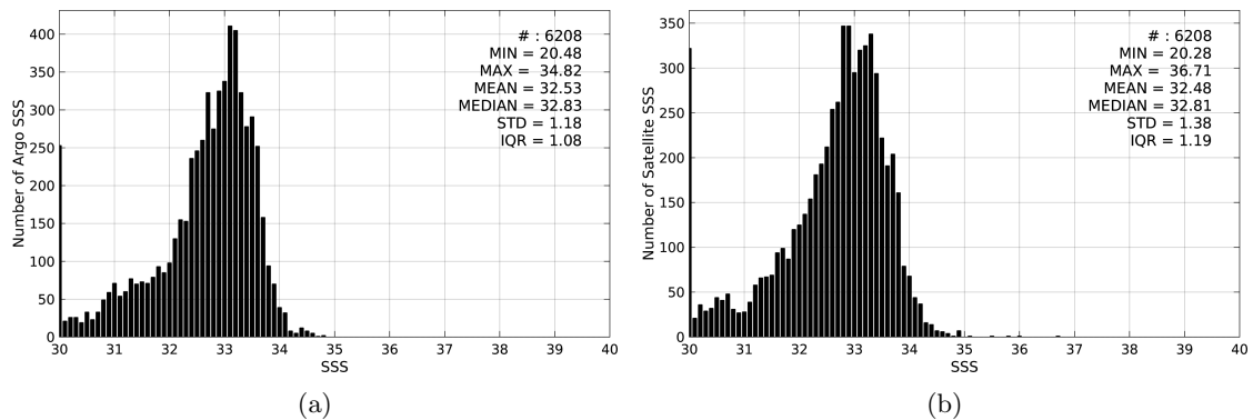
Figure 2: Histograms of SSS from Argo (a) and SMAP-L3-RSS-V2-8DAY-RUNNING-40KM (b) considering all match-up pairs per bins of 0.1 over the Bay of Bengal Pi-MEP region and for the full satellite product period.
