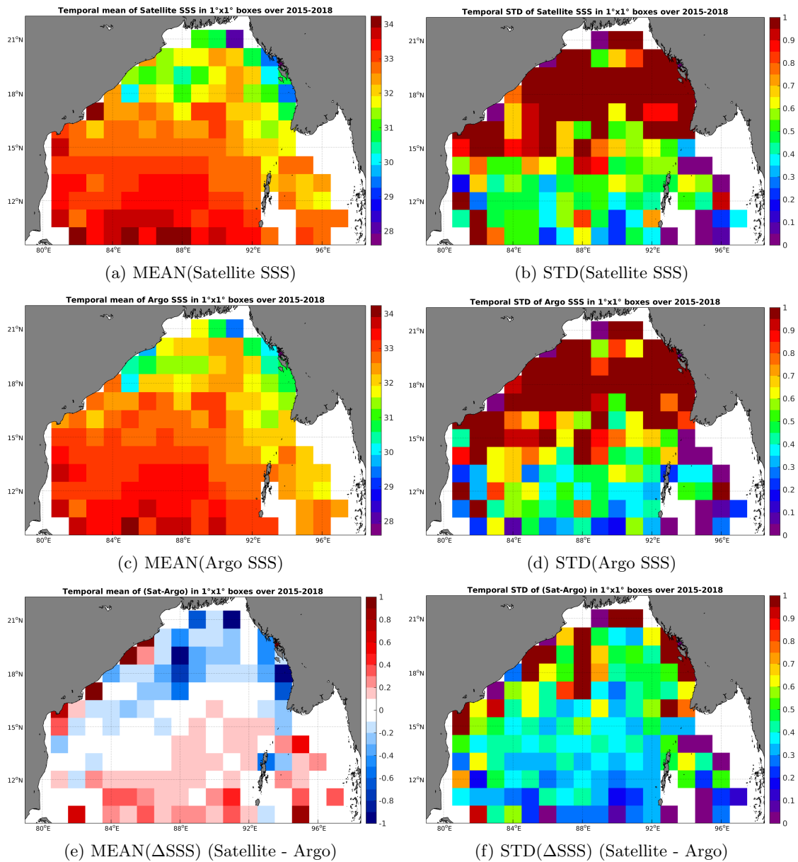
Figure 6: Temporal mean (left) and STD (right) of SSS from SMAP-L3-RSS-V2-8DAY-RUNNING-40KM (top), Argo (middle), and of \Delta SSS (Satellite - Argo). Only match-up pairs are used to generate these maps.
